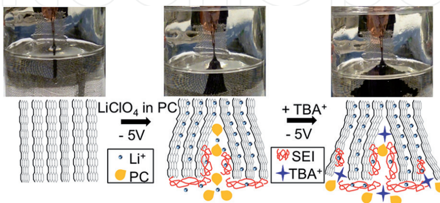
Figure 12. Schematic and images of cathodic electrochemical expansion of graphite.
