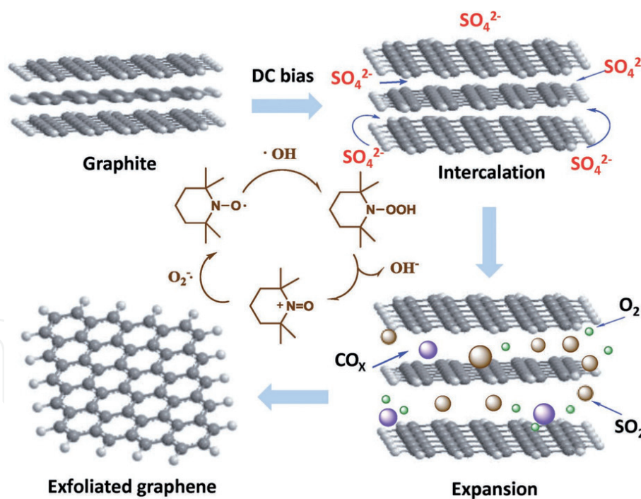
Figure 11. Anodic exfoliation of graphite in an aqueous electrolyte with sulfate anions and TEMPO. TEMPO is a radical scavenger that partially eliminates the hydroxyl radicals from water oxidation [97].
