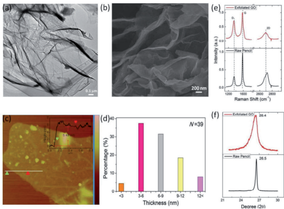
Figure 10. (a) TEM image and (b) SEM image of exfoliated GO flakes, (c) AFM image of exfoliated GO flakes. The thickness is 5.45 nm with lateral size around 2 μm, (d) thickness distribution histograms for exfoliated GO sheets, as estimated from corresponding AFM analysis. The graphene flakes are mainly distributed in the range of 3–9 nm thickness (69%) with lateral size about 1 to few μm, (e) Raman spectra, and (f) XRD patterns for both pencil core and exfoliated GO flakes, respectively [80].
