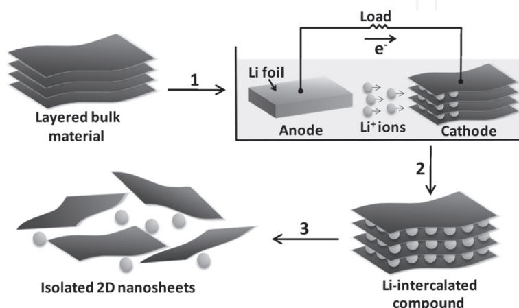
Figure 1. Schematic illustration of electrochemical exfoliation [41].
