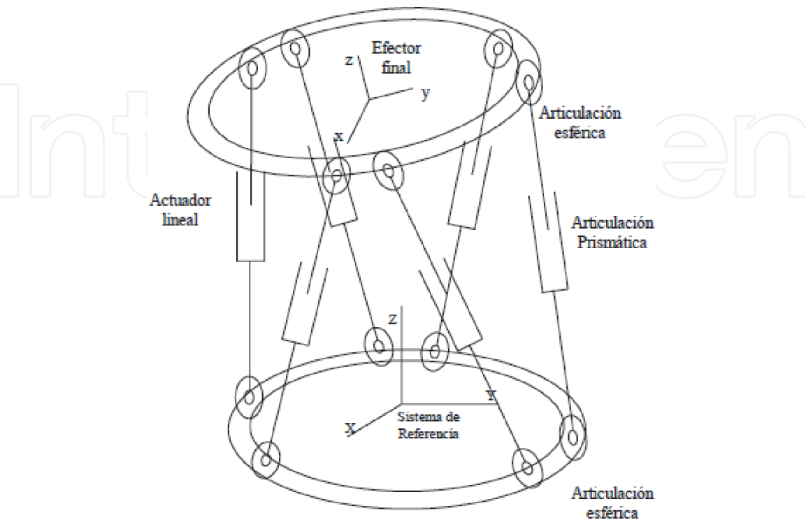
Figure 13. Stewart 6-SPS platform [23].
