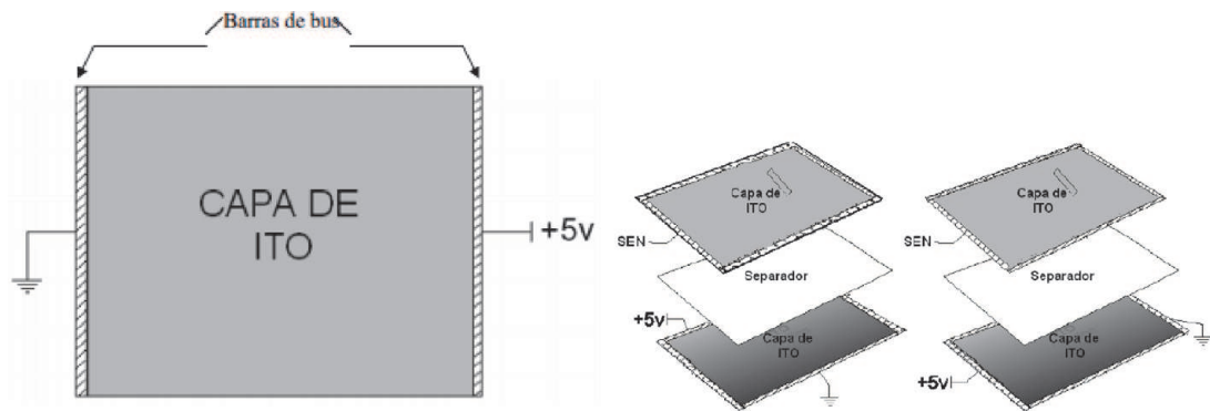
Figure 7. Configuration of the layers of a resistive panel.
