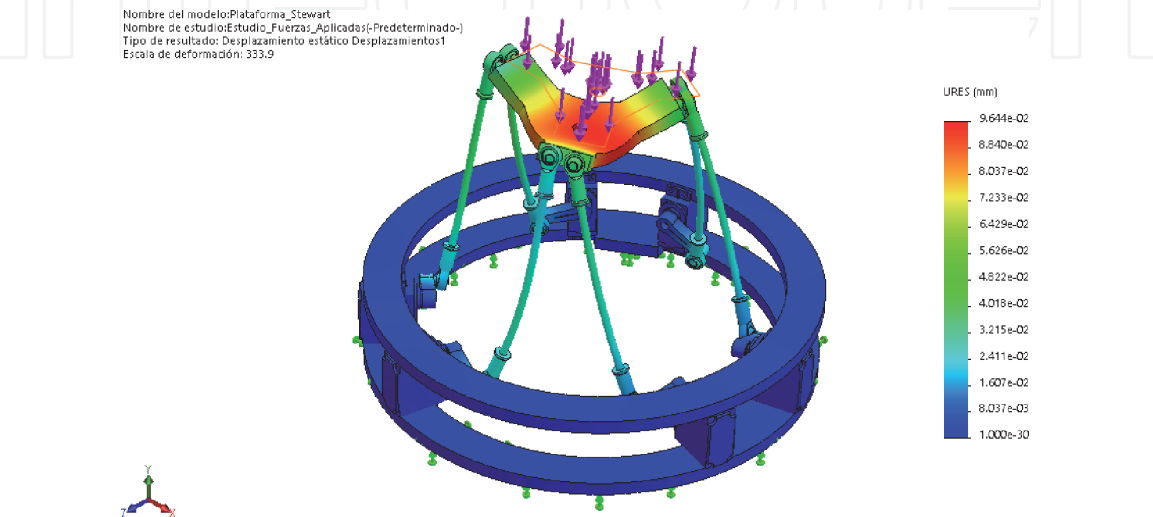
Figure 23. Deformation study.
