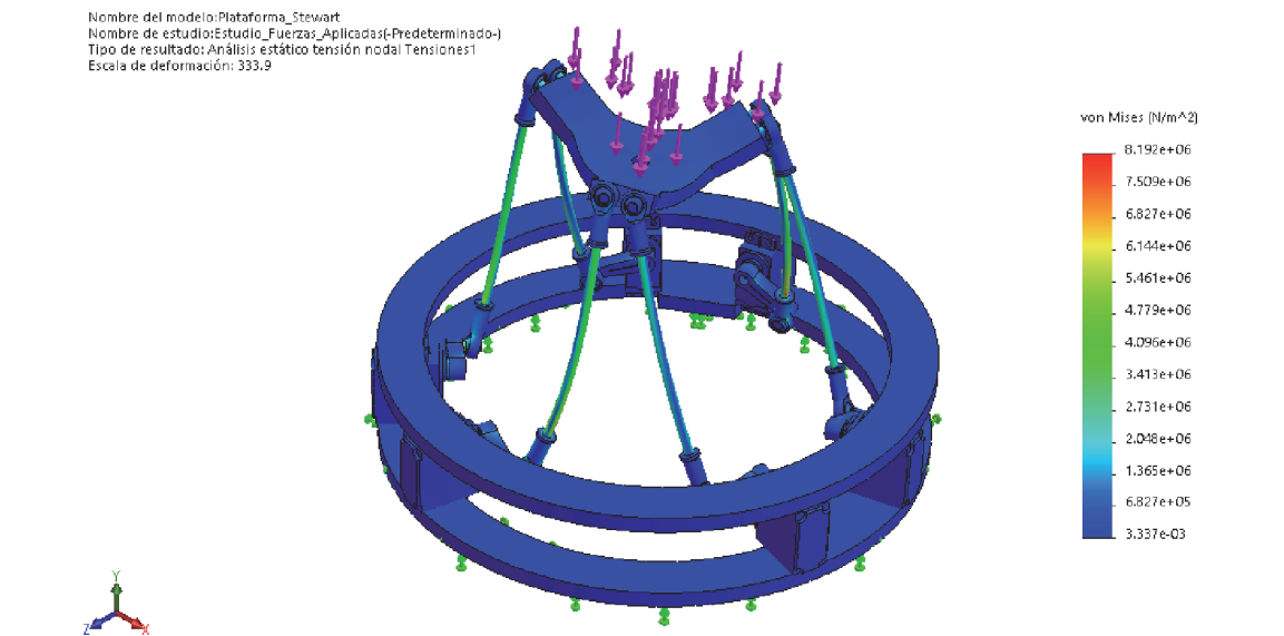
Figure 22. von Mises stress study.
