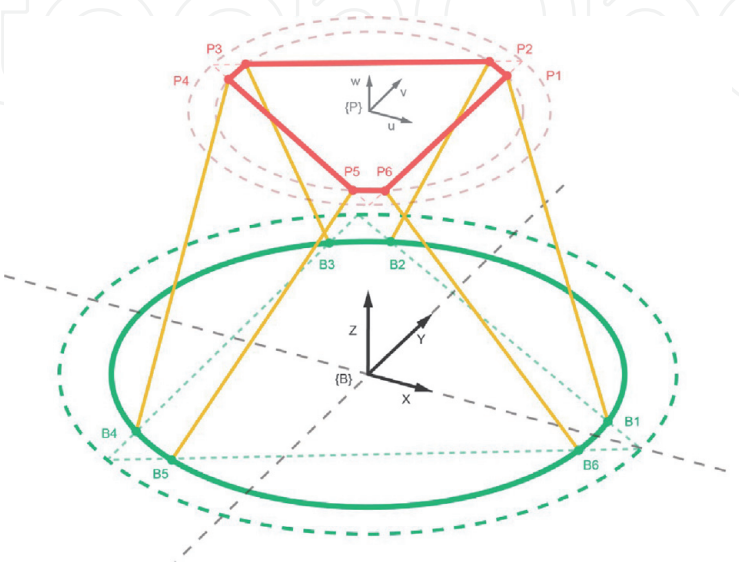
Figure 20. Schematic diagram of new reference systems.
