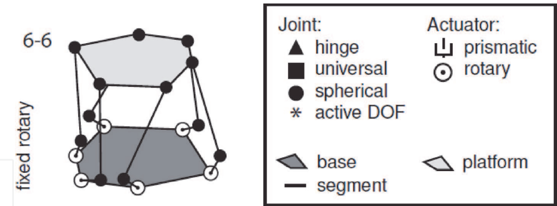
Figure 14. Stewart 6-SPS platform with angular actuators [18].
