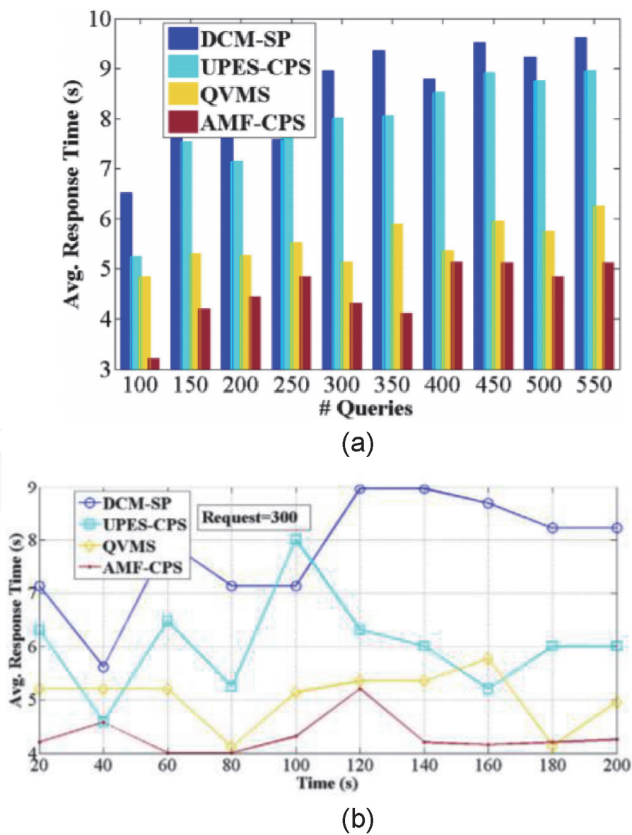
Figure 8. (a). Response time vs. queries. (b). Response time vs. queries.
