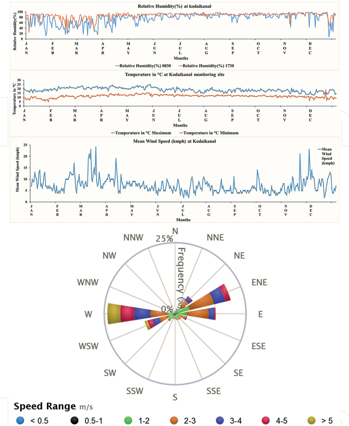
Figure 3. Trends of TGM concentration and meteorological parameters in high-altitude background station (Kodaikanal) in South India.
