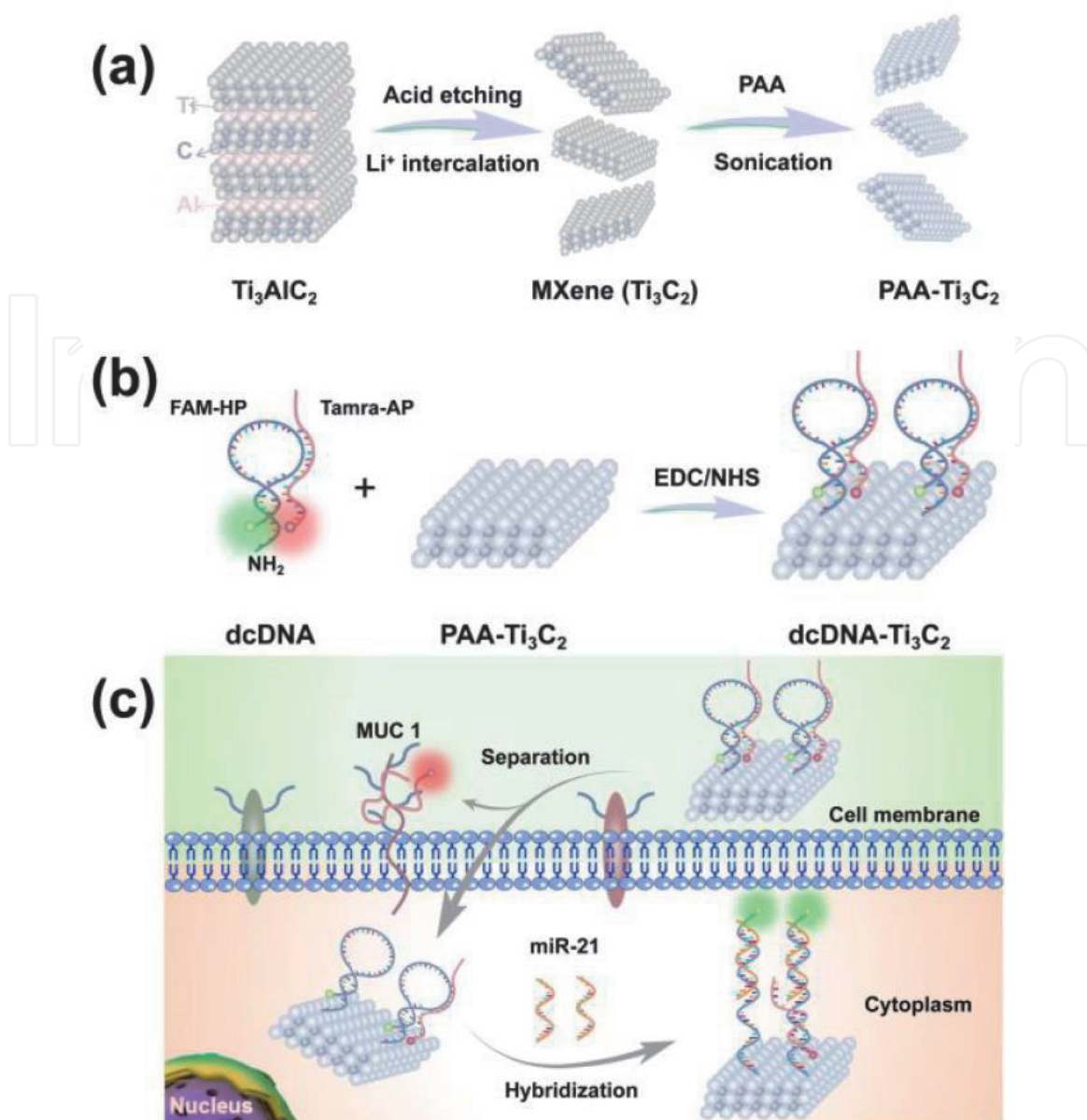
Figure 4. (a) Illustration of the fabrication of the \text{Ti}_3\text{C}_2 MXenes and \text{PAA-Ti}_3\text{C}_2 . (b) the construction of the \text{dcDNA-Ti}_3\text{C}_2 composite nanoprobe. (c) Multilayer imaging of plasma membrane glycoproteins MUC1 and cytoplasmic miR-21 using the \text{dcDNA-Ti}_3\text{C}_2 composite nanoprobe. Reprinted with permission from ref. [128]. Copyright ACS, 2019.
