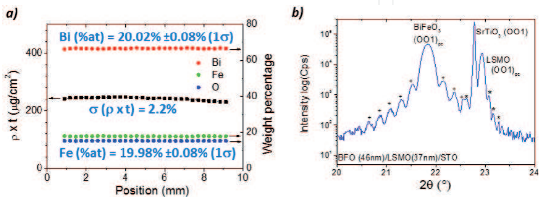
Figure 2. (a) Evolutions of density \times thickness product ( \rho \cdot t ) and weight percentages of Bi, Fe and O as a function of the position (adapted from [18] with permission) and (b) X-ray diffraction pattern of BFO/LSMO/STO heterostructure.
