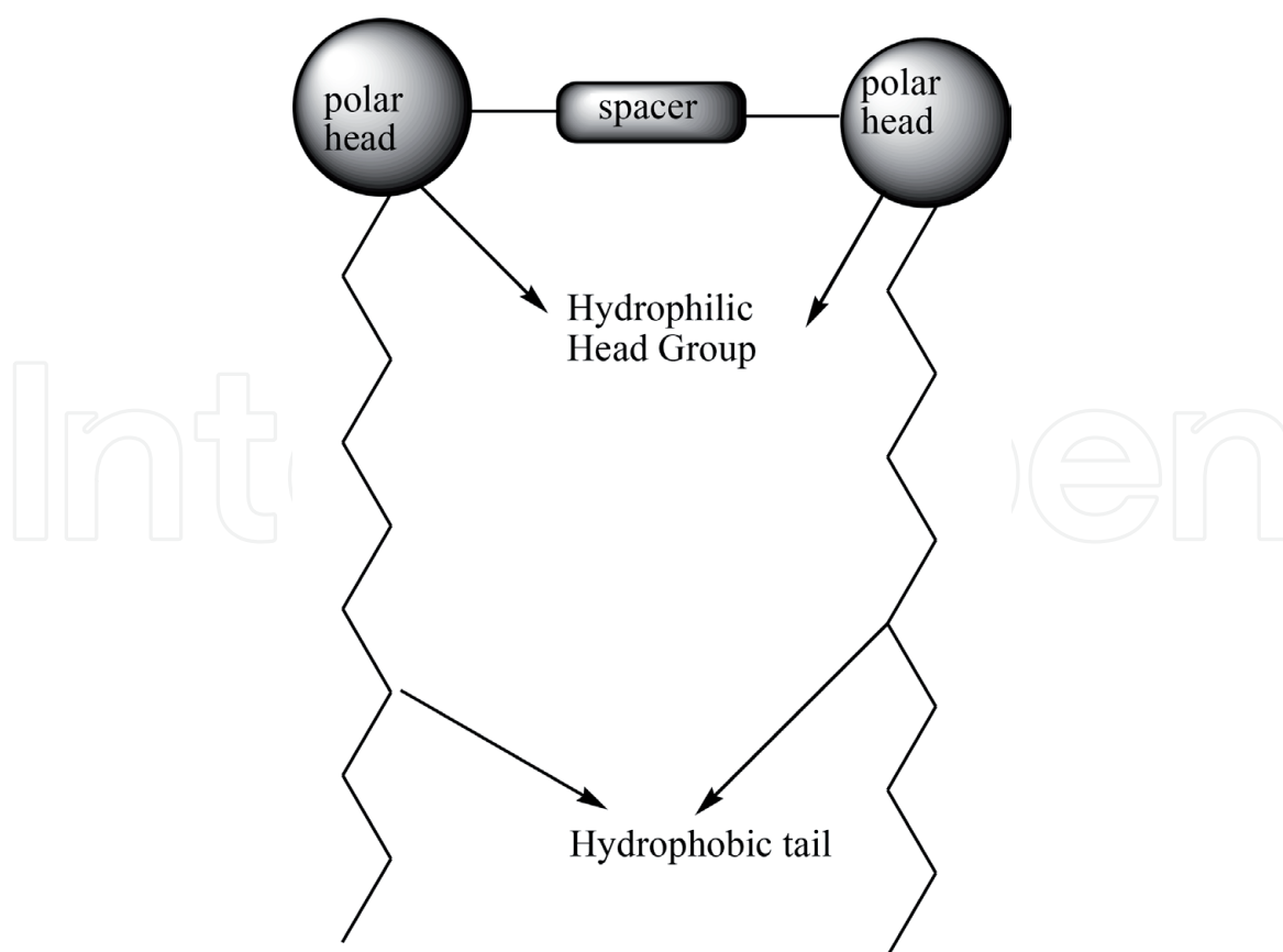
Figure 3. Gemini imidazoline surfactant.
