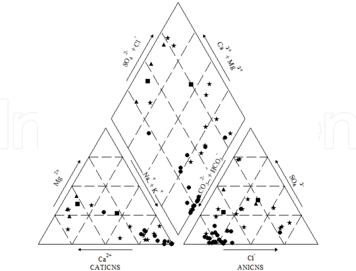
Figure 1. Piper drawing of the ground water (In the figure, the squares stand for surface water, the triangles stand for quaternary water, the circles stand for coal bearing seam water, and the stars stand for limestone aquifer water).
