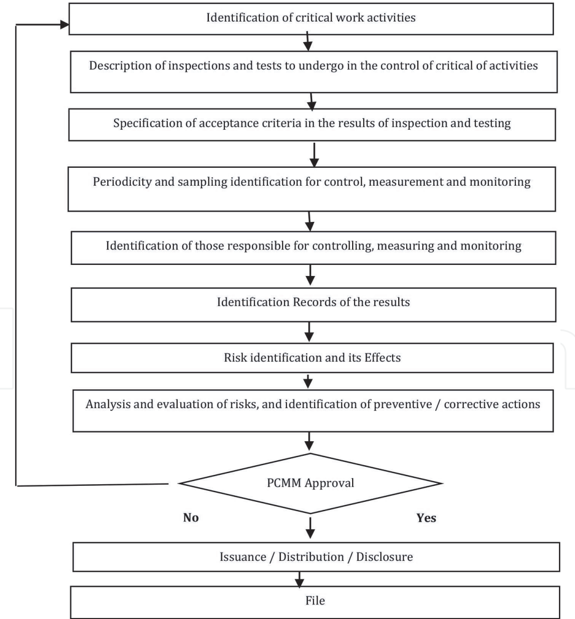
Figure 1. Flowchart for preparing PCMM [2].
