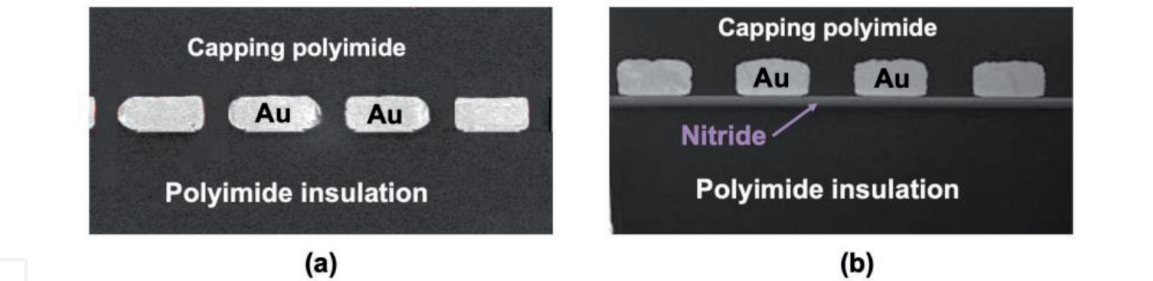
Figure 13. Isolation transformer without (a) and with SiN charge injection barrier (b).
