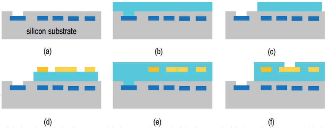
Figure 3. Isolation transformer process flow. (a) CMOS substrate with top metal, (b) polyimide layer spin coated, (c) polyimide layer patterned & cured, (d) top coil plated, (e) 2 nd polyimide layer spin coated and (f) 2 nd polyimide layer patterned & cured.
