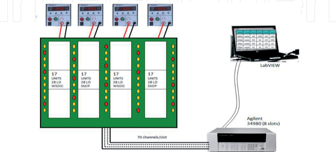
Figure 8. Experimental setup for high voltage endurance test.
