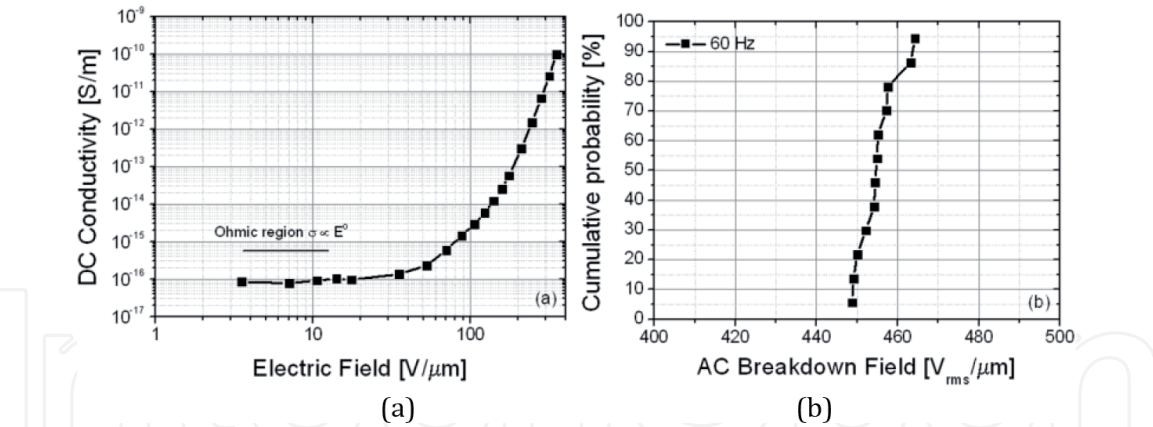
Figure 6. Main intrinsic electrical properties of spin-coated polyimide films measured at wafer level: (a) DC conductivity versus electric field and (b) AC breakdown field distribution.
