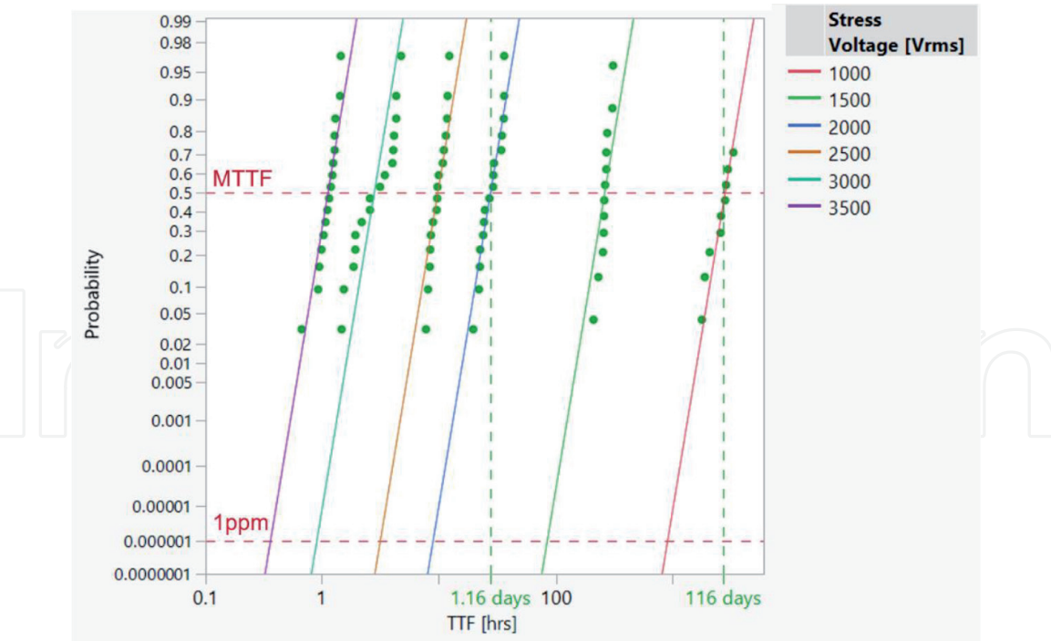
Figure 9. Weibull distribution for isolators with 20-μm thick polyimide.
