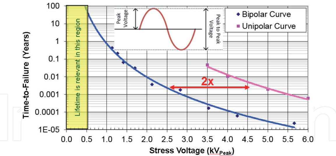
Figure 12. Time-to-failure comparisons for AC bipolar versus unipolar.
