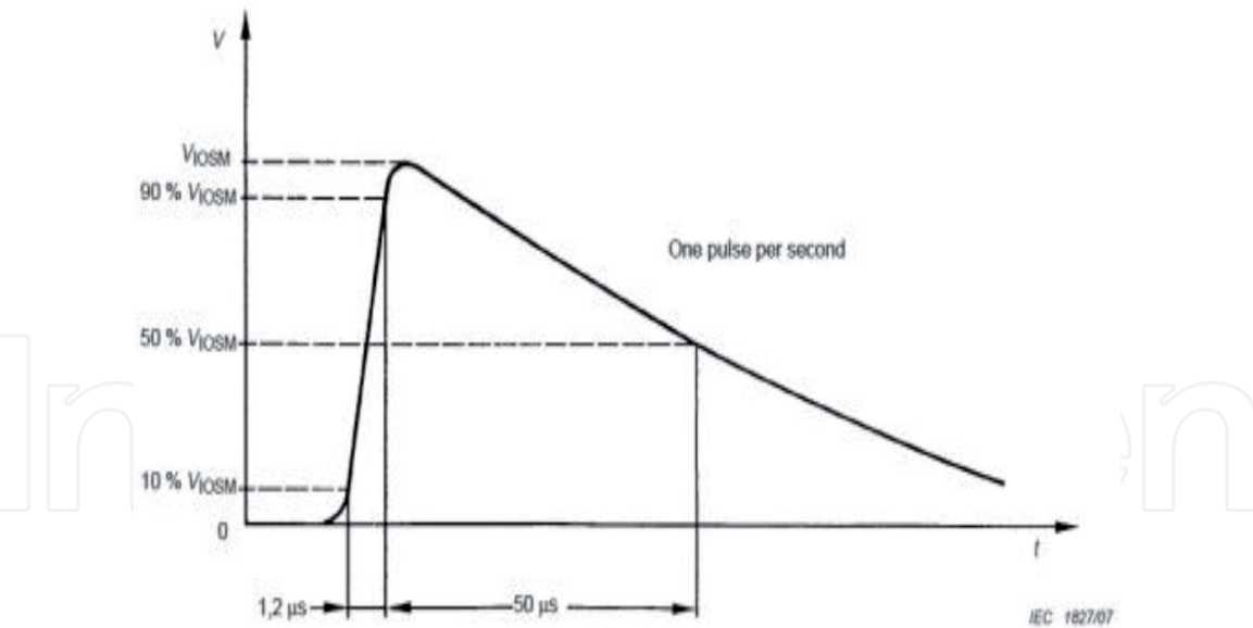
Figure 5. IEC61010-1 Surge test waveform.
