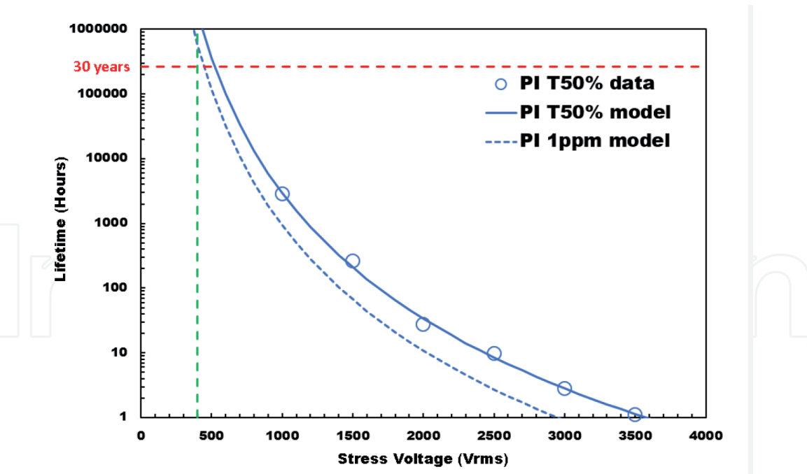
Figure 10. Time-to-failure plot for isolators with 20-μm thick polyimide.
