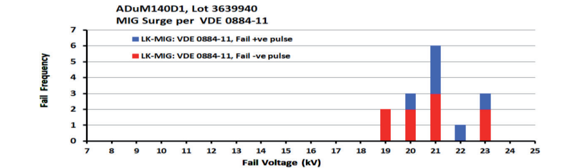
Figure 7. Surge performance for isolators with polyimide films 30 μm thick.
