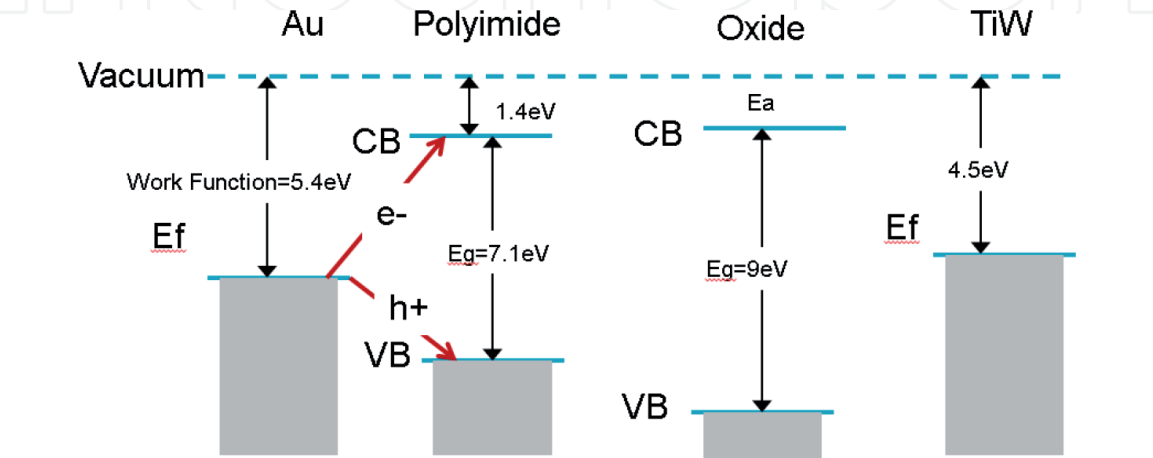
Figure 14. Band diagram for charge injection.
