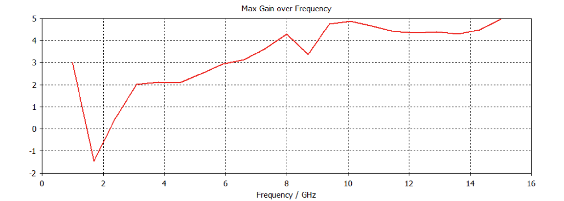
Figure 9. Gain diagram of circular patch antenna.
