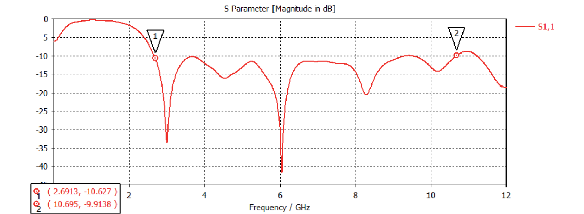
Figure 21. Return loss of array antenna.
