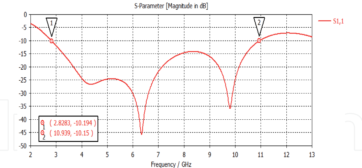
Figure 2. The return loss S_{11} as a function of frequency.
