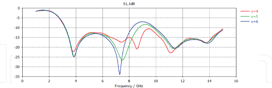
Figure 18. Return loss with effect of the antenna slot location.
