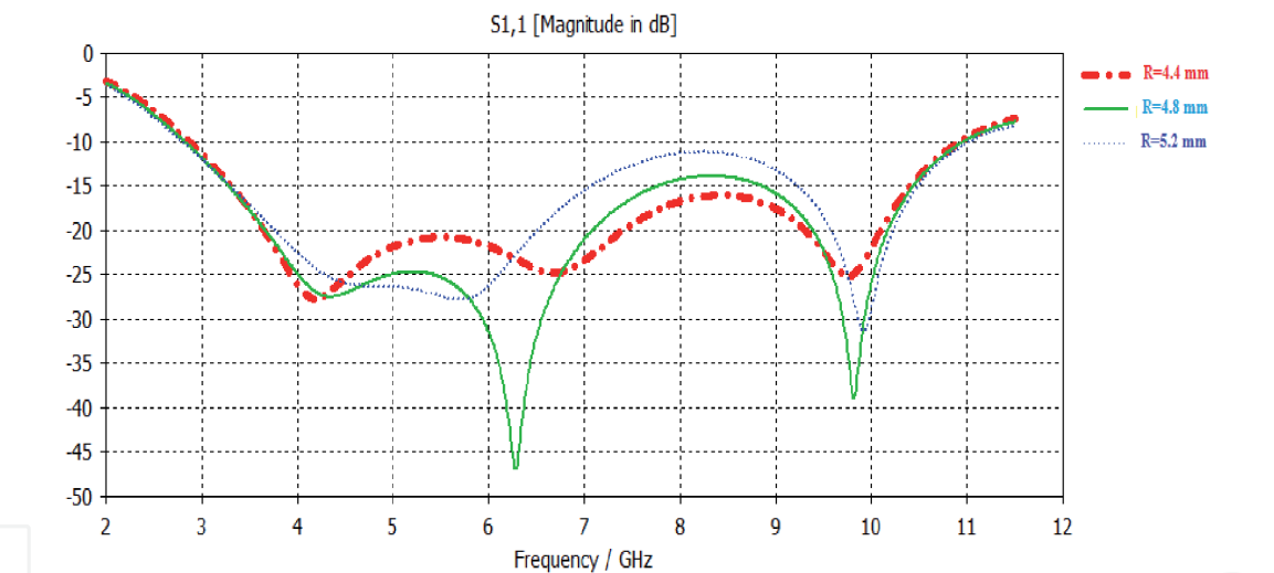
Figure 6. Effect of the inner radius on the antenna.
