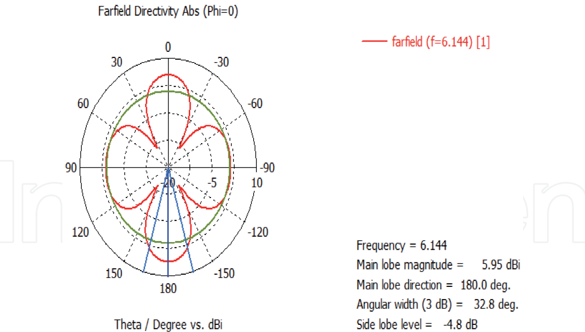
Figure 26. Farfield directivity.
