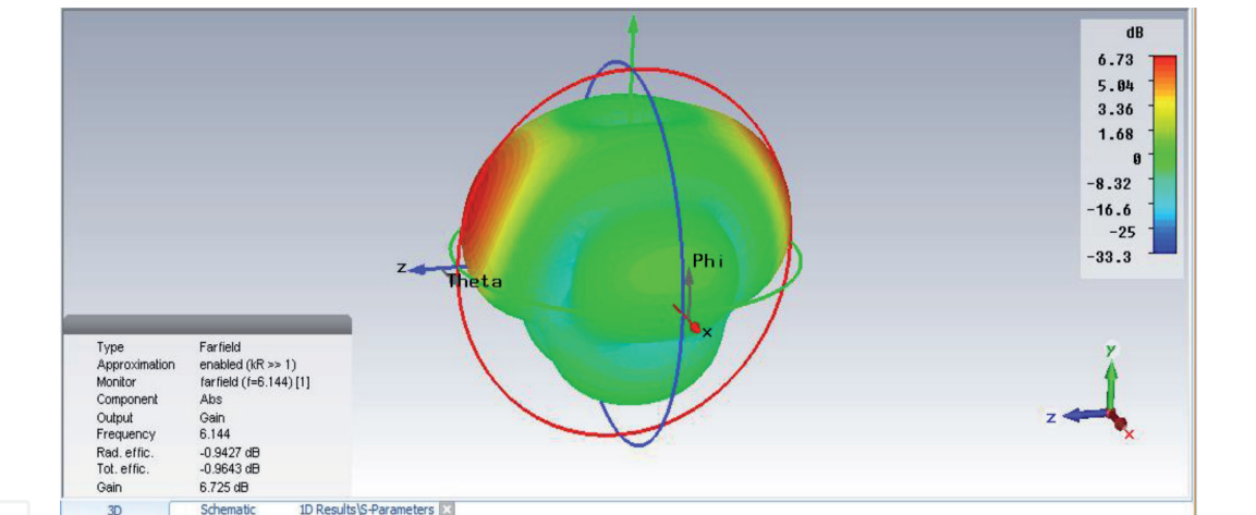
Figure 23. Gain diagram of array antenna.
