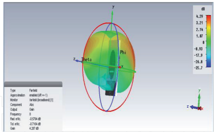
Figure 10. Gain diagram (3D) of circular patch antenna.
