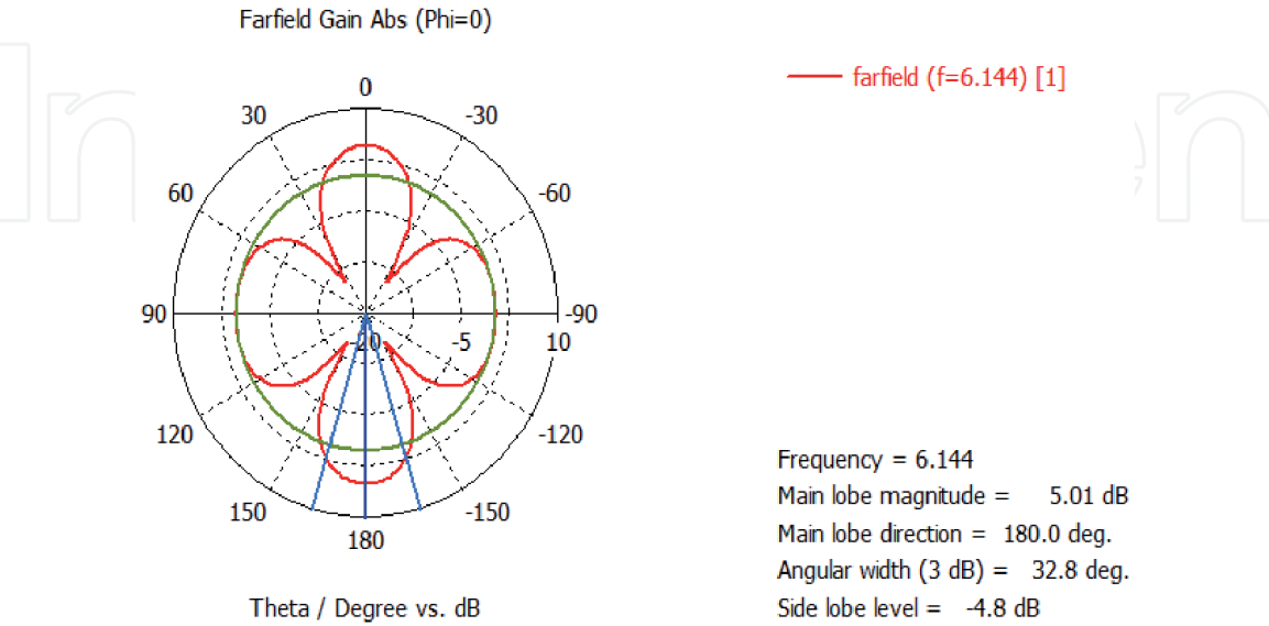
Figure 25. Farfield gain.
