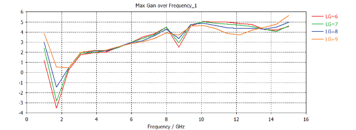
Figure 17. Gain diagram with effect of length of the antenna ground plane.
