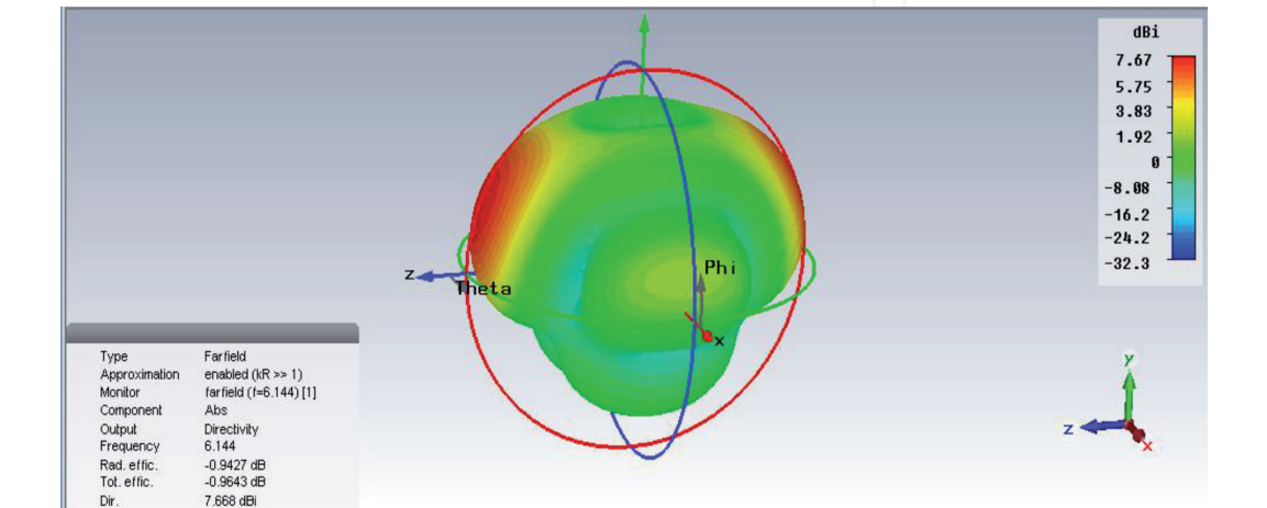
Figure 24. Directivity diagram.
