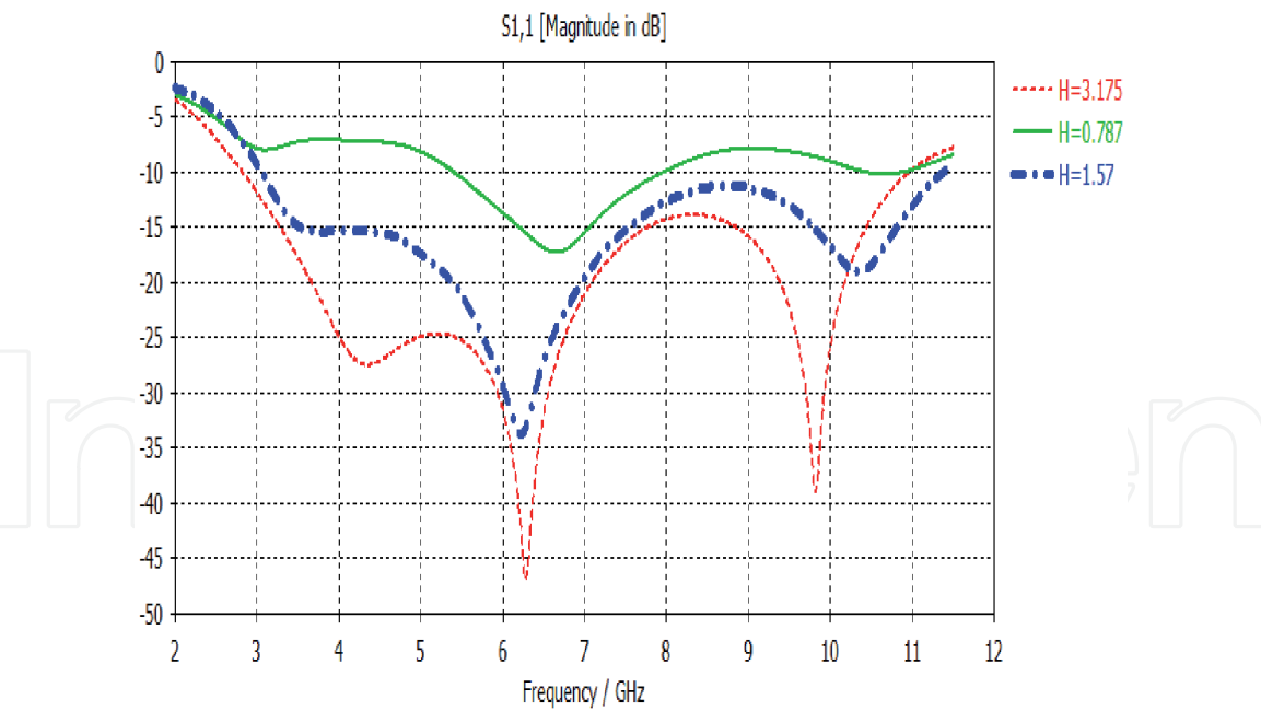
Figure 5. Effect of the thickness of the substrate.
