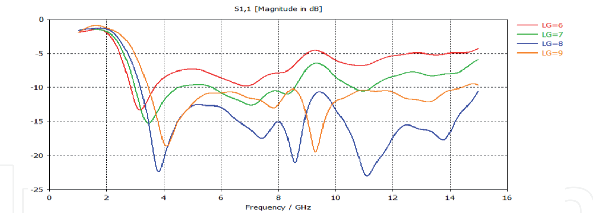
Figure 16. Return loss with effect of the length of the antenna ground plane.
