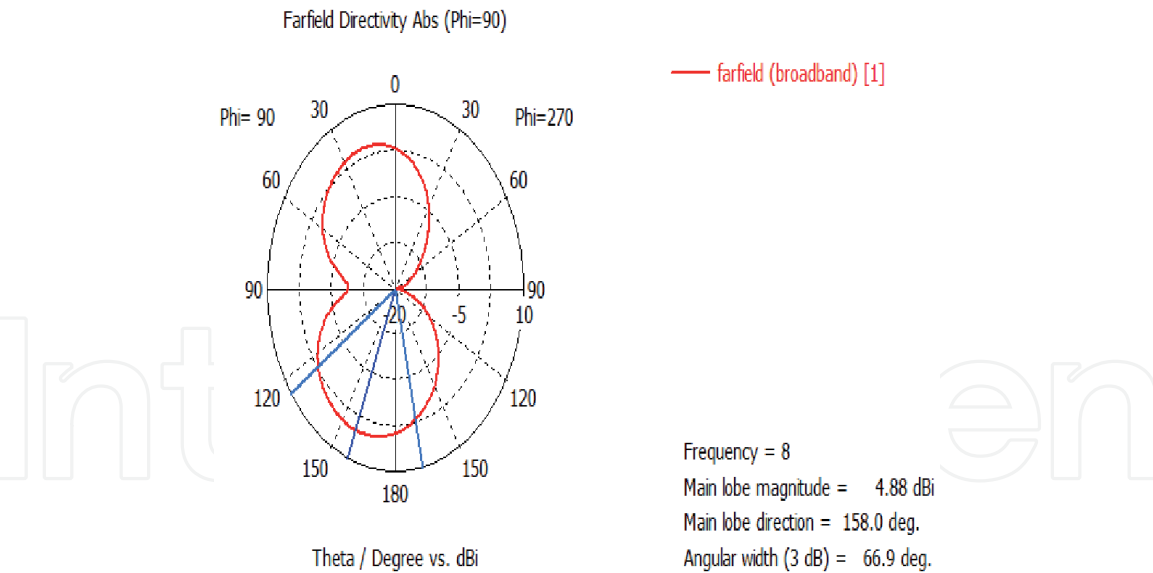
Figure 13. Far-field directionality (2D).
