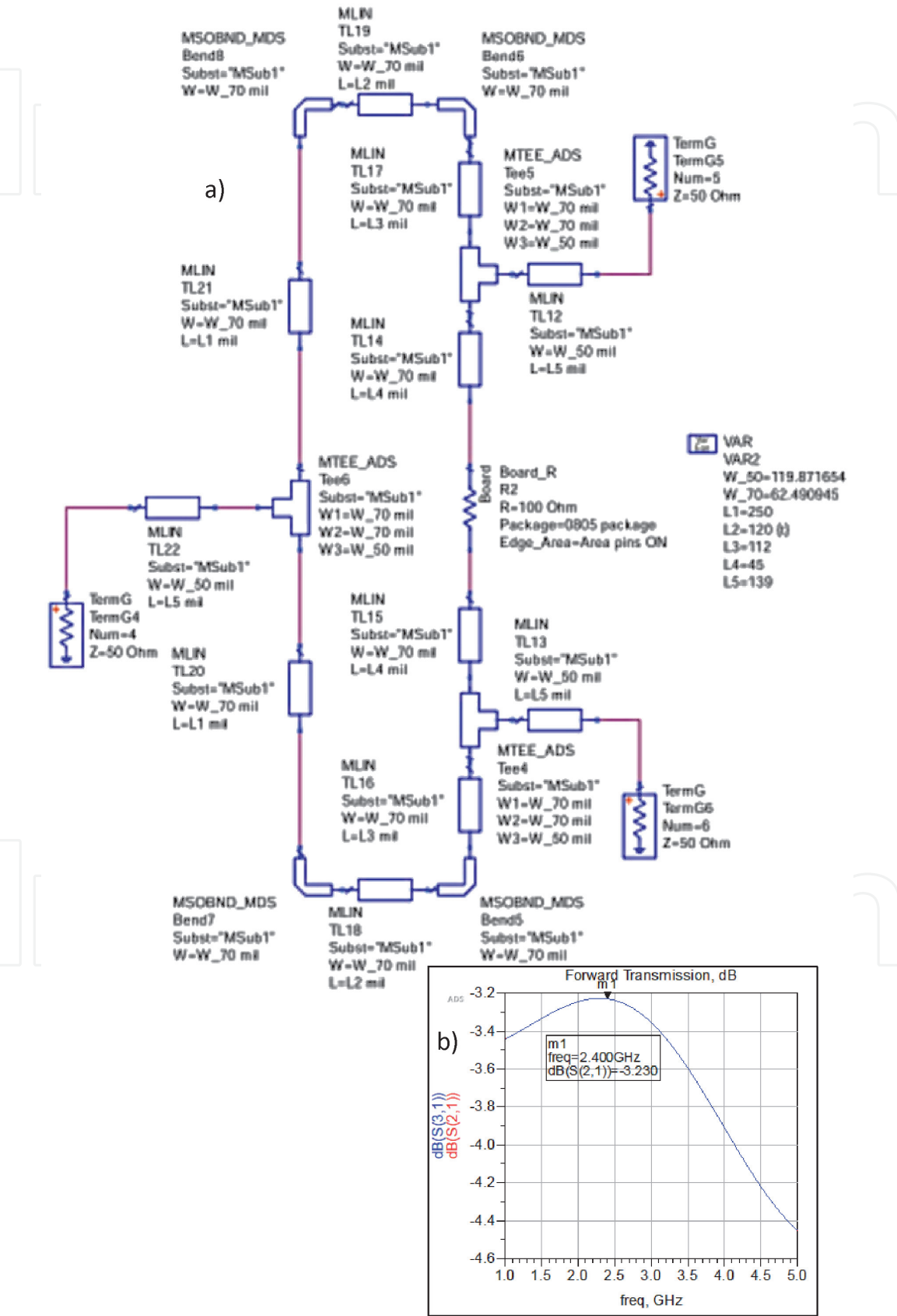
Figure 19. The 2-way WPD: (a) schematic circuit; (b) forward gains S_{21} , S_{31} .
