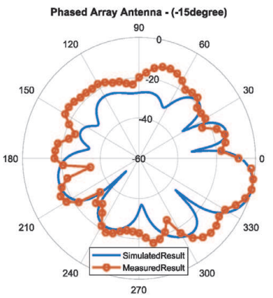
g) Radiation pattern at -15° angle
