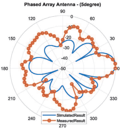
b) Radiation pattern at 5° angle
