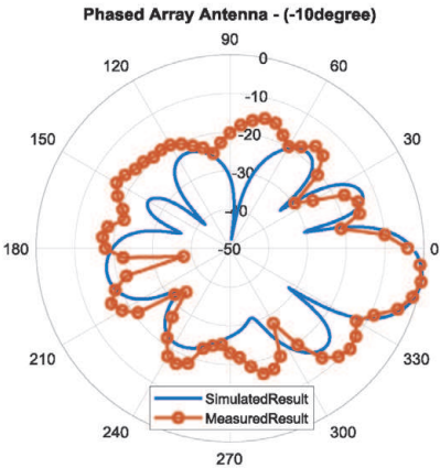
e) Radiation pattern at -10° angle
