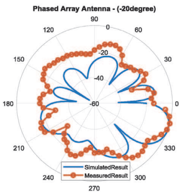
i) Radiation pattern at -20° angle
