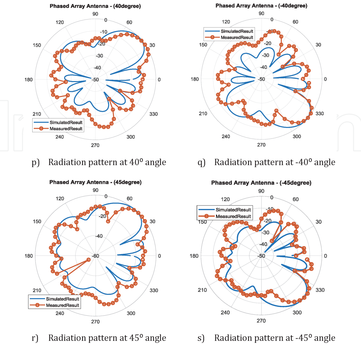
Figure 33. Radiation pattern of phased array antenna at different angles.
