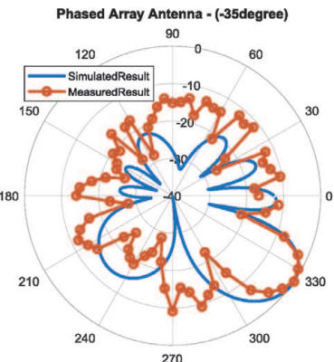
o) Radiation pattern at -35° angle
