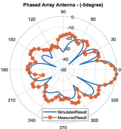
c) Radiation pattern at -5° angle
