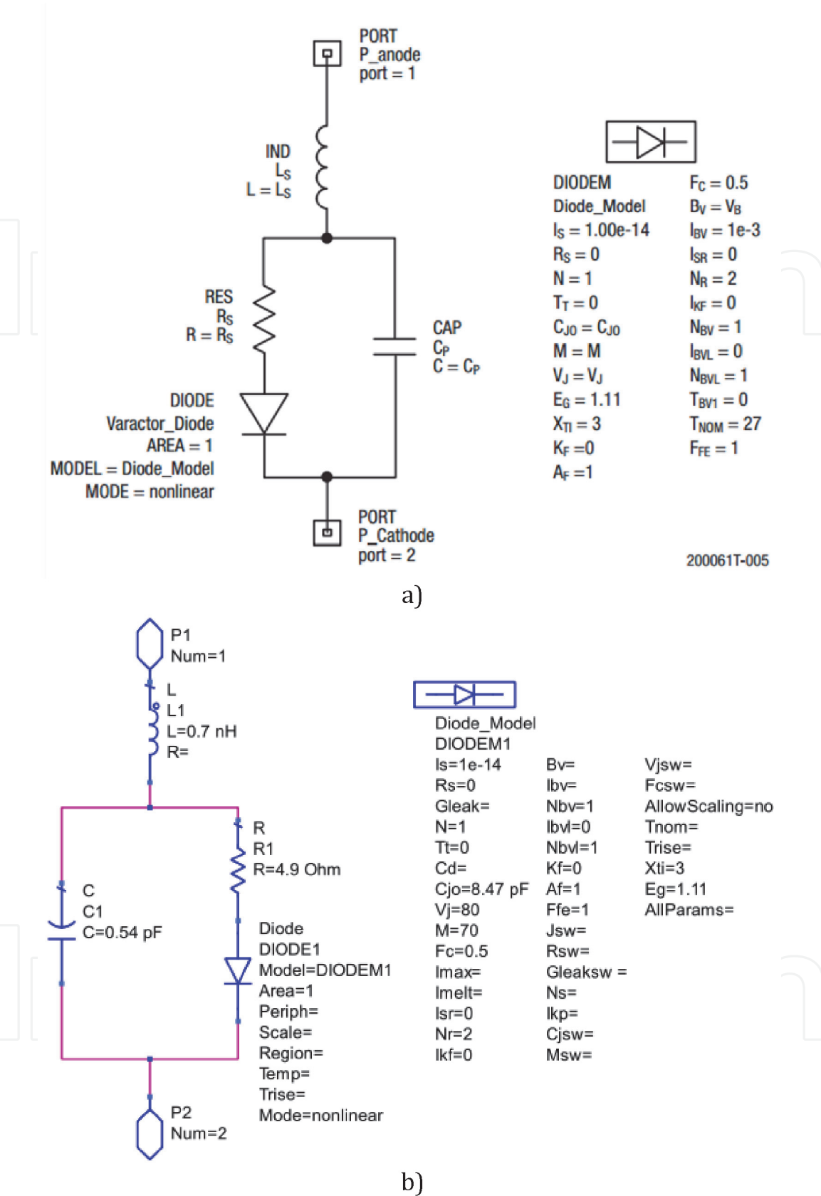
Figure 24. Equivalent model of SMV1247: (a) on SPICE [36]; (b) on ADS.
