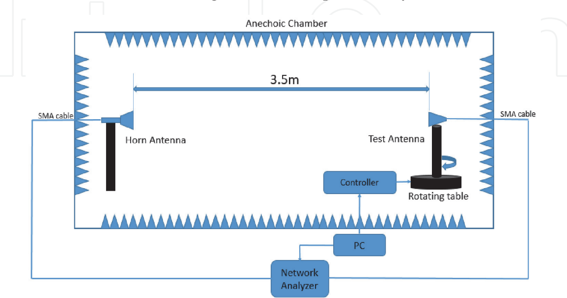
Figure 30. Anechoic chamber configuration for measuring beamforming antenna array.
