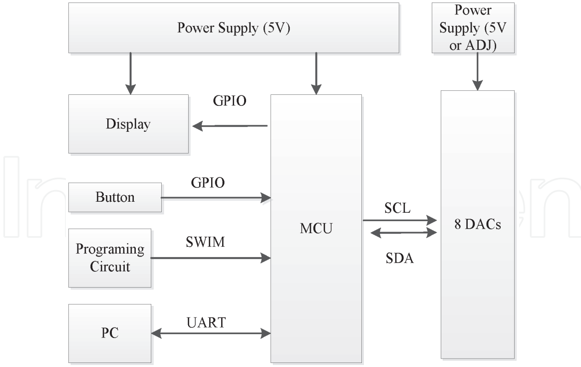
Figure 17. Block diagram of varactor diode controller.
