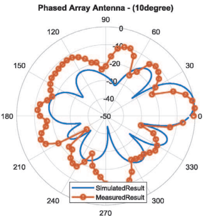
d) Radiation pattern at 10° angle
