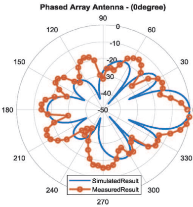
a) Radiation pattern at 0° angle
