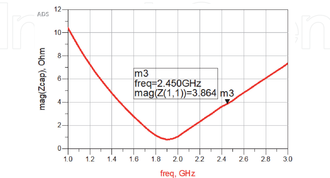
Figure 16. Impedance of DC block VJ0603D8R2CXP.
