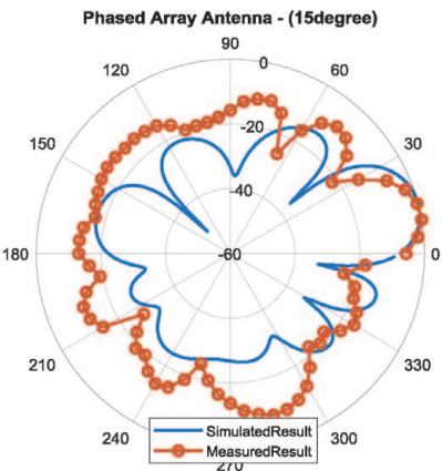
f) Radiation pattern at 15° angle
