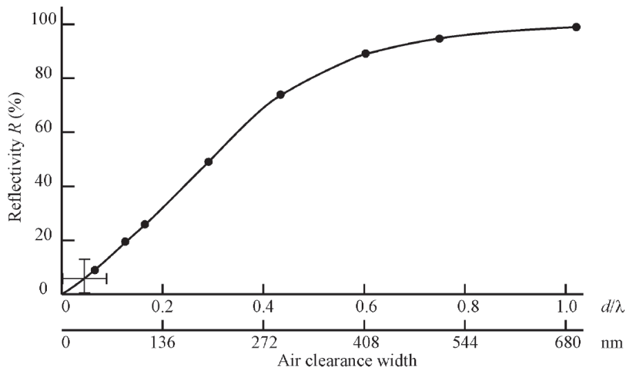
Figure 6. Experimental data presented the relationship between the waveguide slit width and the reflectivity magnitude are obtained by AITR method. The point characterized the slitless collimator has a specific design.
