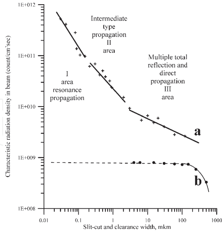
Figure 9. Experimental dependences of CuK \alpha \beta flux radiation densities on slit width for X-ray beams formed by PXWs (a) and by the single slit-cut system (b).
