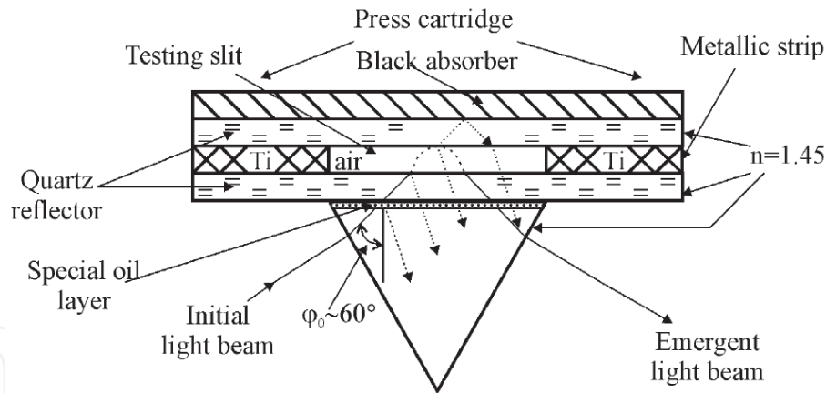
Figure 5. Principle scheme for direct measurements of a waveguide slit width by methods of the attenuated internal total reflection (AITR). I and II are quartz reflectors of a waveguide. Scheme was published, in first, in Ref. [34].
