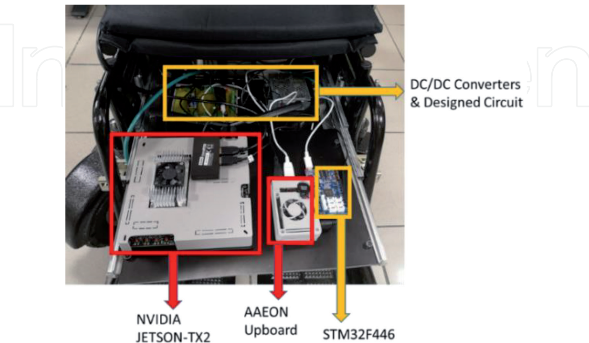
Figure 4. Computational hardware of autonomous wheelchair (drawer is open).
