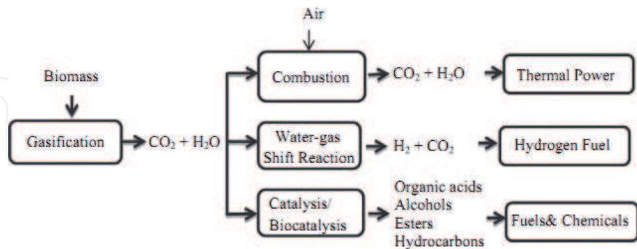
Figure 19. Transformation processes of biomass into products by gasification [19].
