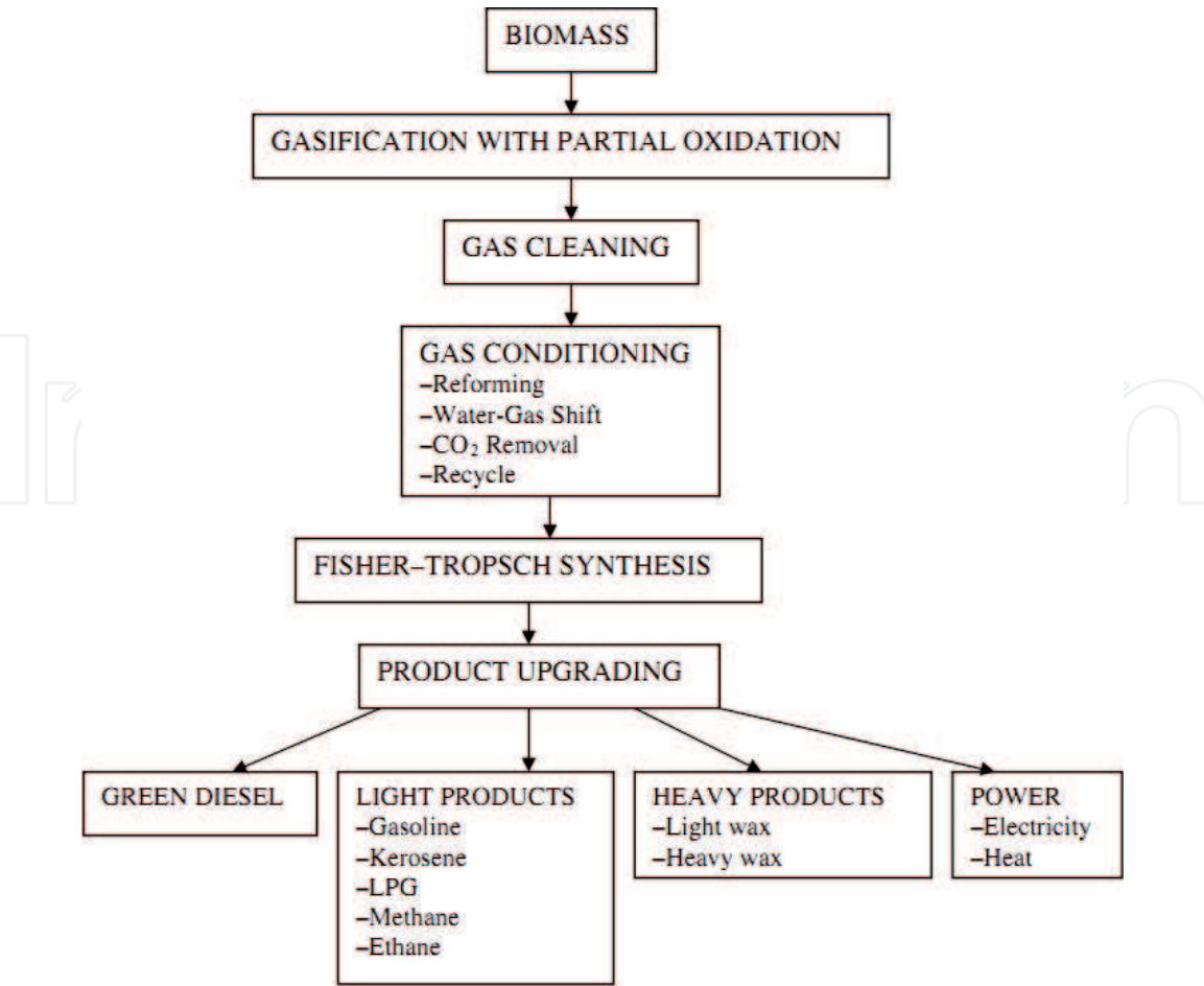
Figure 20. Products obtained from biomass by Fischer-Tropsch synthesis [20].
