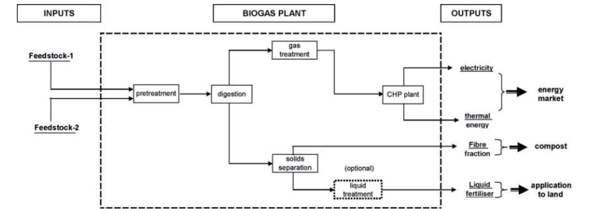
Figure 22. Flow diagram of the biogas production facility [24].
