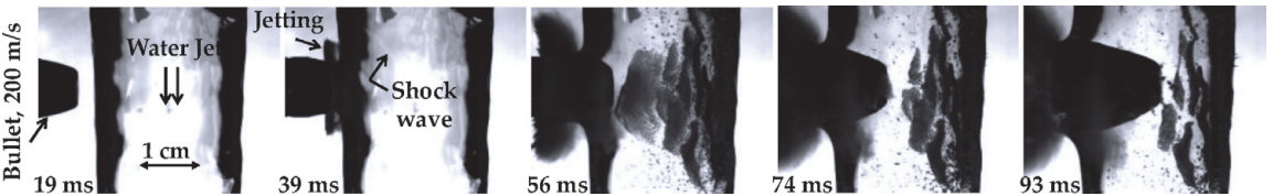
Figure 8. Visualization of a high-speed impact of a 9 mm bullet on a \sim 2 cm water jet. Evidence of secondary cavitation due to shockwaves confinement.
