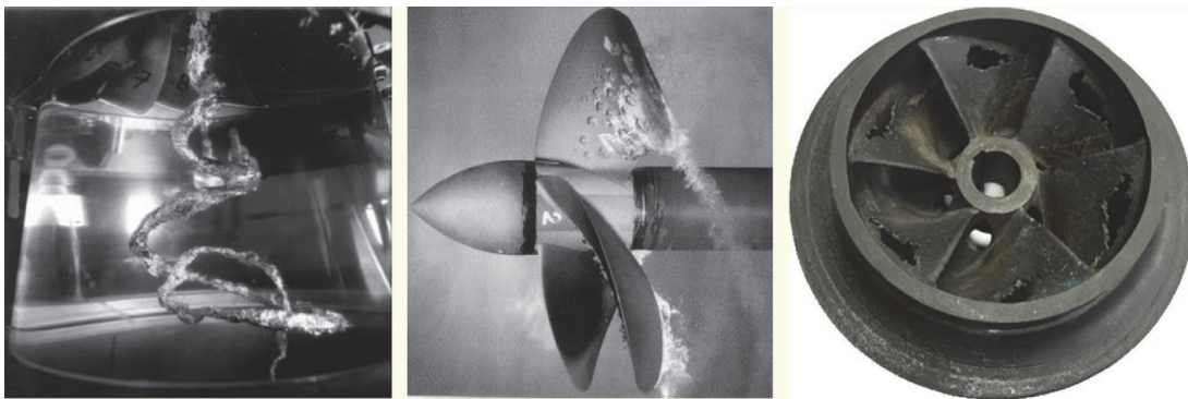
Figure 1. Left: cavitating vortex in a Francis turbine, operating at off-design conditions; middle: cavitation in a ship propeller (courtesy Franc et al. [4]); right: pump impeller heavily eroded by cavitation.
