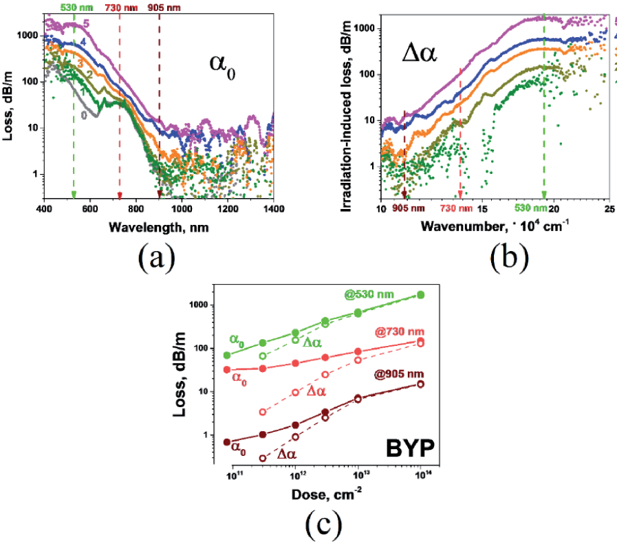
Figure 9. (a) Attenuation spectra ( \alpha_0 ) in VIS/NIR vs. wavelength and (b) IA spectra ( \Delta\alpha ) vs. wavenumber for BYP fiber in pristine state (curves “o”) and after growing \beta -irradiation dose (curves “1” to “5”). (c) Dose dependences of small-signal absorption ( \alpha_0 , solid curves) and IA ( \Delta\alpha , dashed curves), measured at wavelengths 905, 730, and 530 nm.
