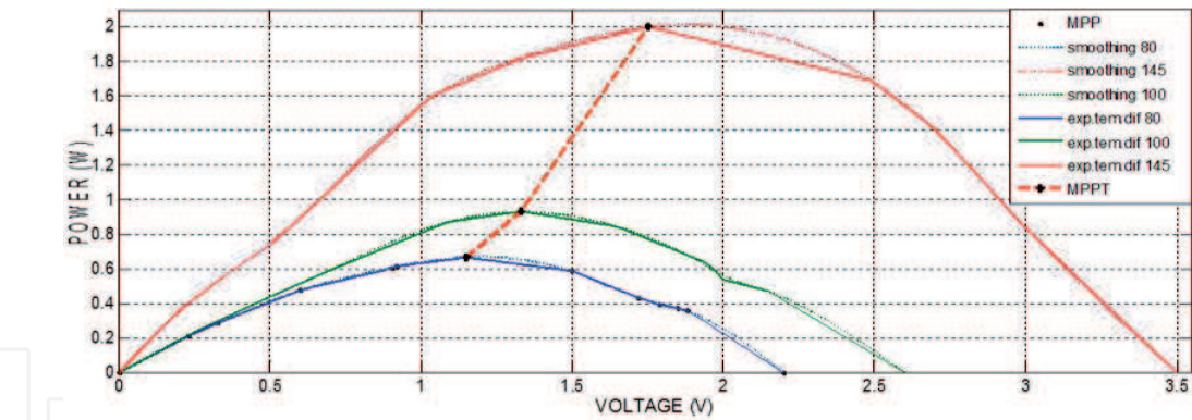
Figure 9. P-I characterization of TEG mode (TEP1-142T300) for three different \Delta T .
