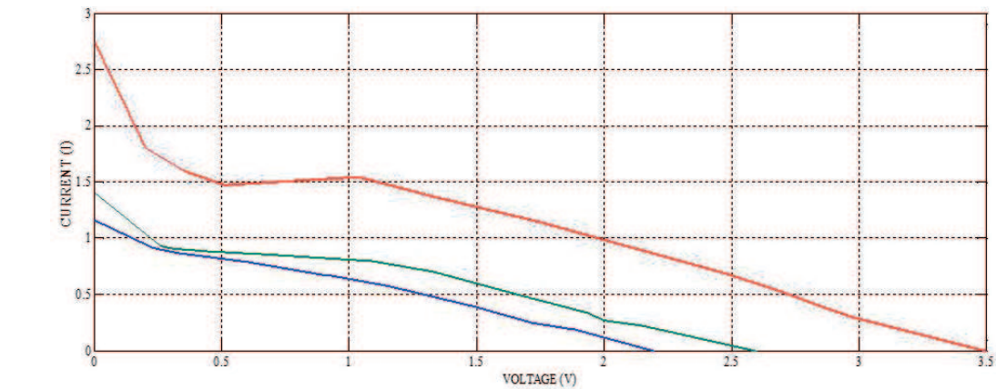
Figure 10. V-I characterization of TEG mode (TEP1-142T300) for three different \Delta T .
