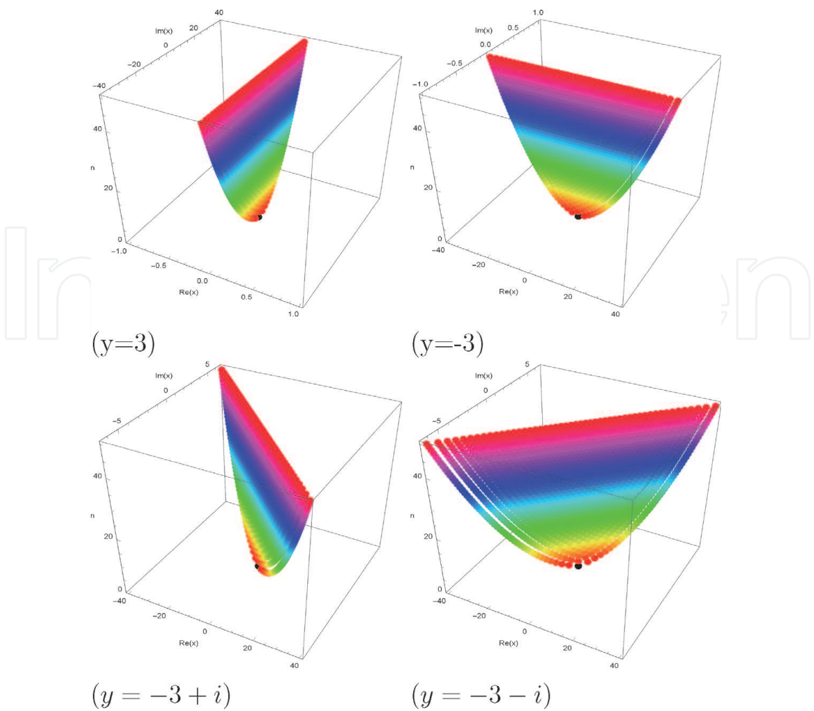
Figure 3. Stacks of zeros of H_n(x,y|\mu) = 0, 1 \leq n \leq 50 .
