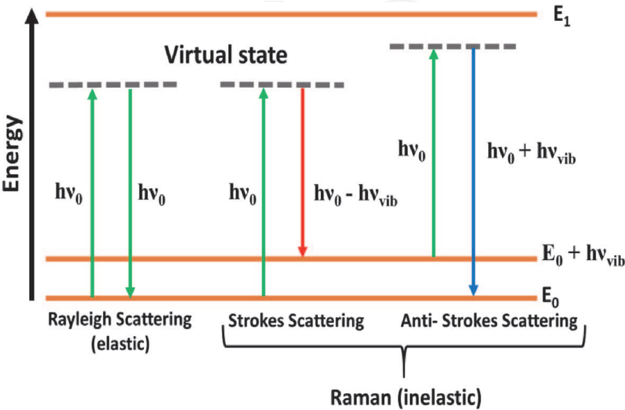
Figure 1. Energy level diagram for Rayleigh and Raman scattering, where \Delta E = h\nu_{vib} represents the difference in vibration energy levels [7].
