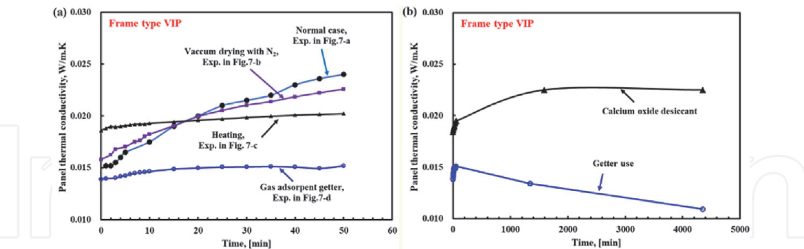
Figure 20. Variation of the center-of-panel thermal conductivity with the elapsed time for (a) different trial manufacturing methods and (b) two different outgassing adsorbent materials [6].
