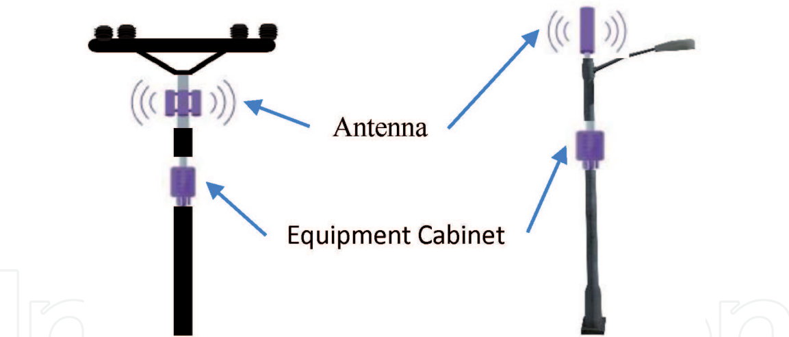
Figure 1. Small cells mounted on power pole and streetlights.
