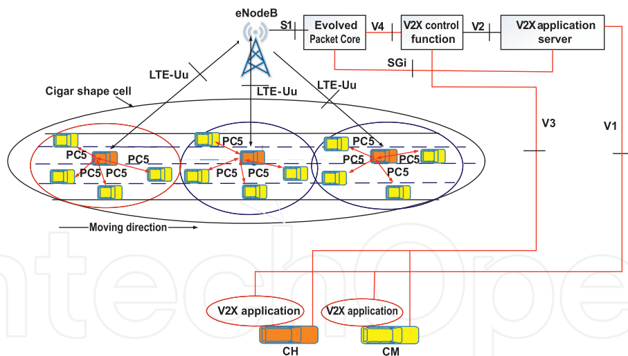
Figure 8. Highway scenario for proposed cluster-based V2V cellular (CBC-V2V) architecture.
