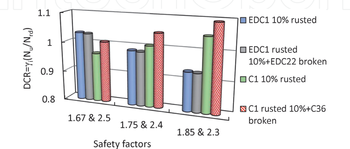
Figure 11. Effect of corrosion and, combined effect of cable loss and corrosion on DCR of C1 and EDC1.
