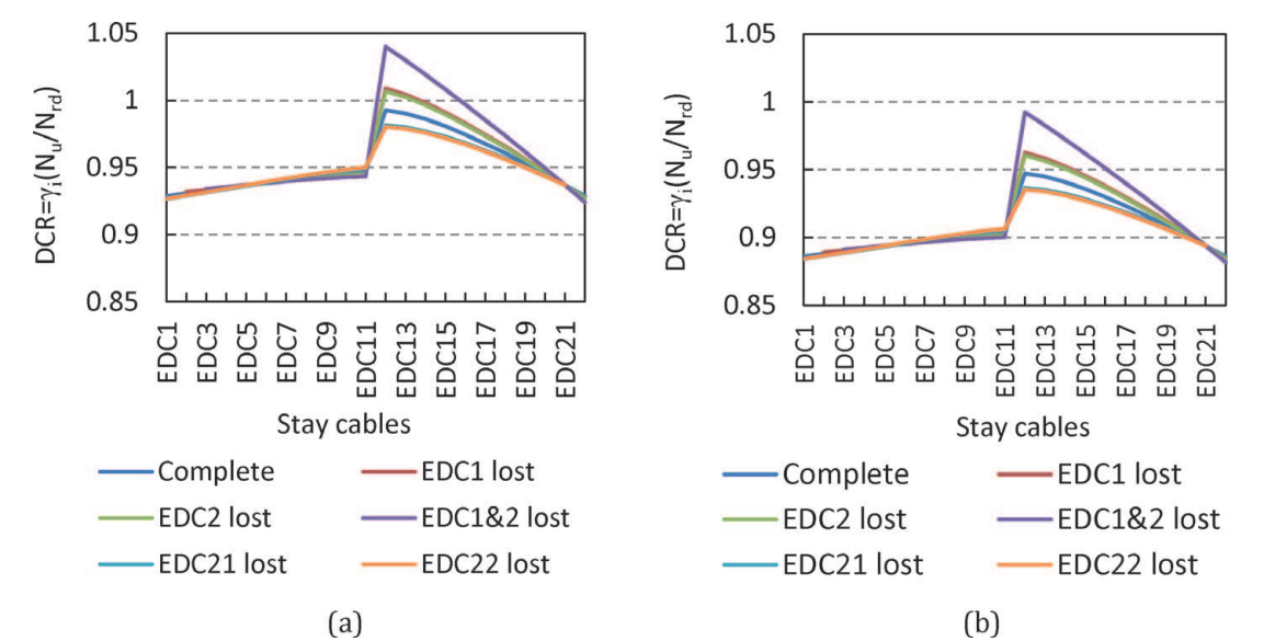
Figure 10. Effect of cable loss on DCR of stay cables of extradosed bridge. (a) Safety factor of 1.67 and (b) safety factor of 1.75.
