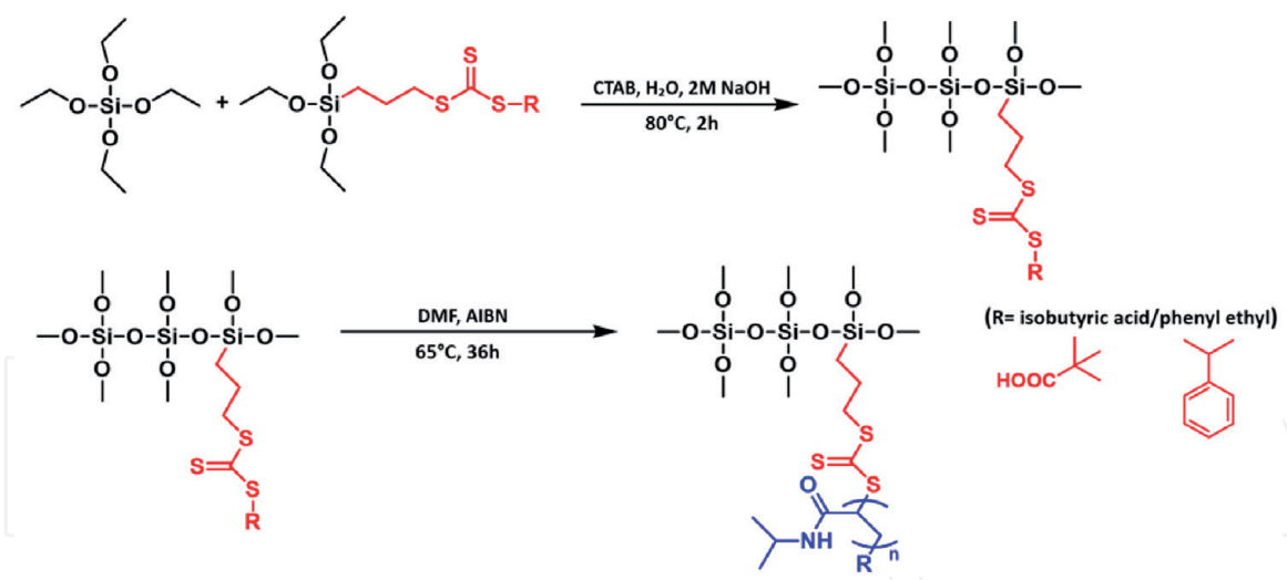
Figure 6. Schematic representation for MSNs functionalized with different R group containing organoalkoxysilane RAFT agent via co-condensation and further grafting with PNIPAM via surface-initiated RAFT polymerization as reported by Mishra et al. (reproduced with permission from Ref. [31]).
