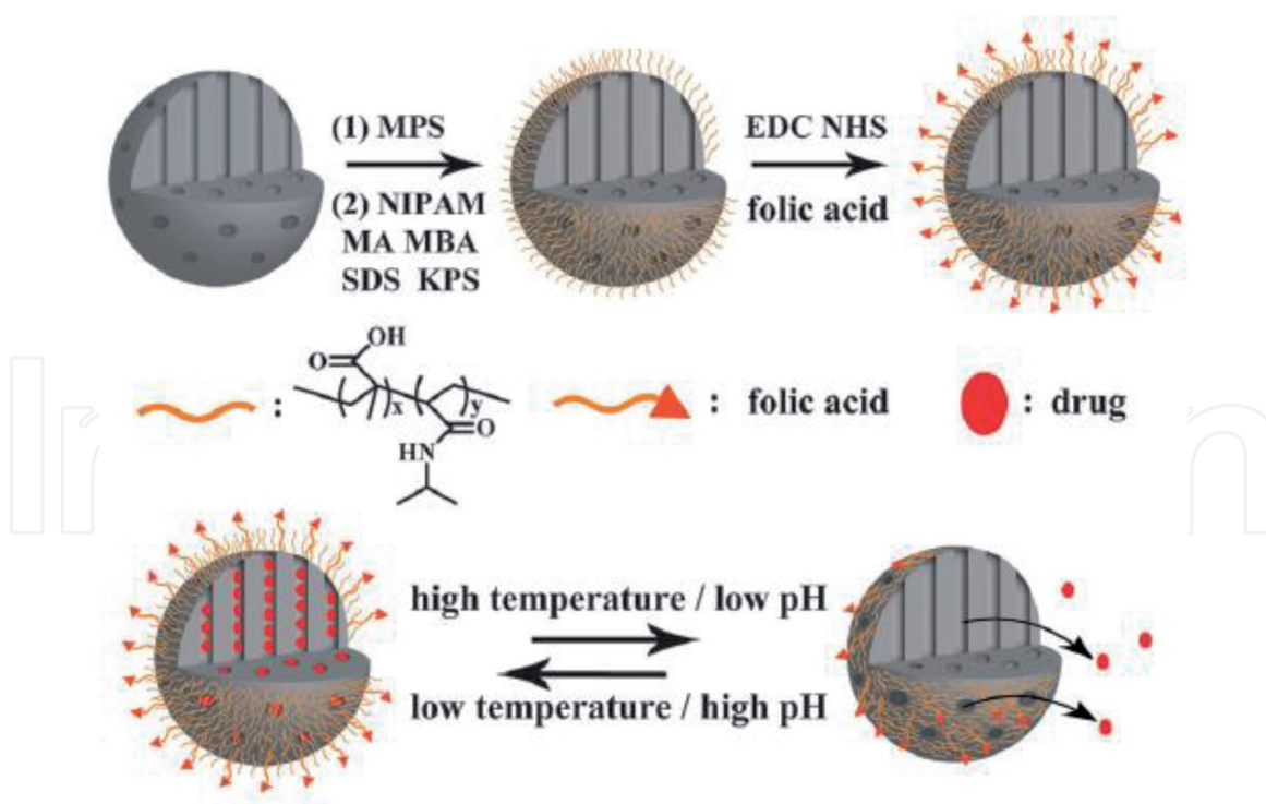
Figure 14. Illustration of synthesis of dual-responsive drug delivery system (reproduced with permission from Ref. [47]).
