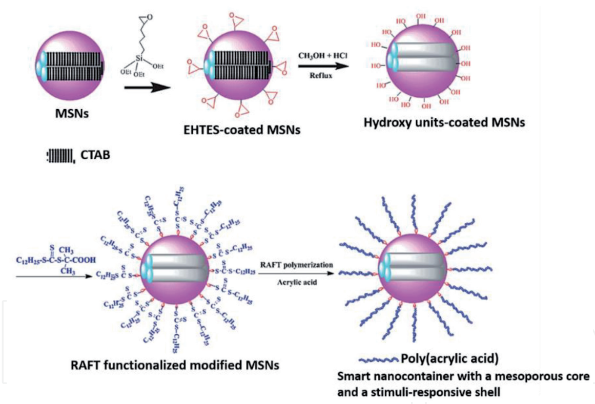
Figure 7. Schematic representation for grafting of poly(acrylic acid) on the exterior surface of MSNs via RAFT polymerization as reported by Hong et al. (reproduced with permission from Ref. [33]).
