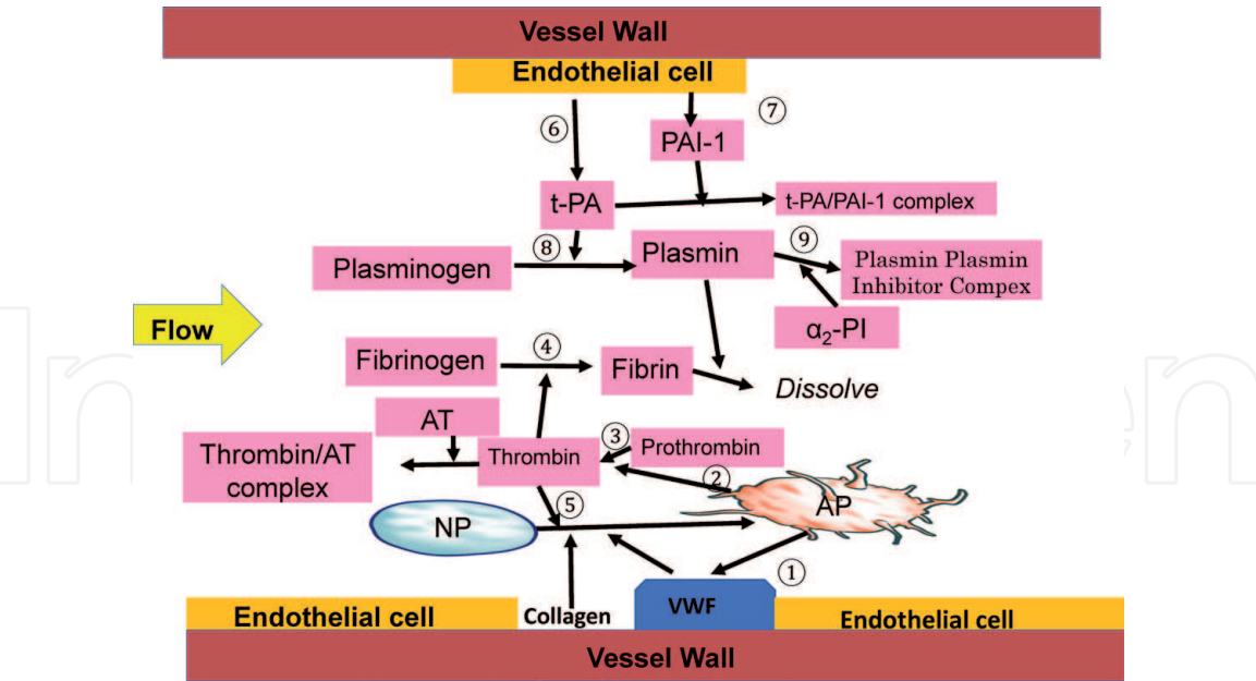
Figure 4. Coupling model of blood flow, platelet, coagulation, and fibrinolysis. Thrombus formation at the site of endothelial injury is modeled. Nonactivated platelets (NP) adhered at the site of endothelial injury through von Willebrand factor (VWF) and collagen are exposed there. NP become activated platelets (AP) by their interaction with VWF/collagen (①). AP has a potential to convert prothrombin to thrombin on their membrane surface (②). After production of thrombin from prothrombin (③), thrombin converts soluble fibrinogen to fibrin thrombi. (④) thrombin also has a function to further activate platelets through thrombin receptor stimulation. (⑤) Fibrinolytic system is also incorporated in this model. Functional endothelial cells constitutively release both tissue-type plasminogen activator (t-PA: ⑥) and plasminogen activator inhibitor (PAI)-1 (⑦). T-PA converts plasminogen to plasmin, which has fibrinolytic activity (⑧) unless inactivated by binding with PAI-1. Plasmin is a strong enzyme able to degrade fibrin. Its function is immediately neutralized by its binding with \alpha_2 -plasmin inhibitor to form plasmin \alpha_2 -plasmin inhibitor complex (PIC: ⑨).
