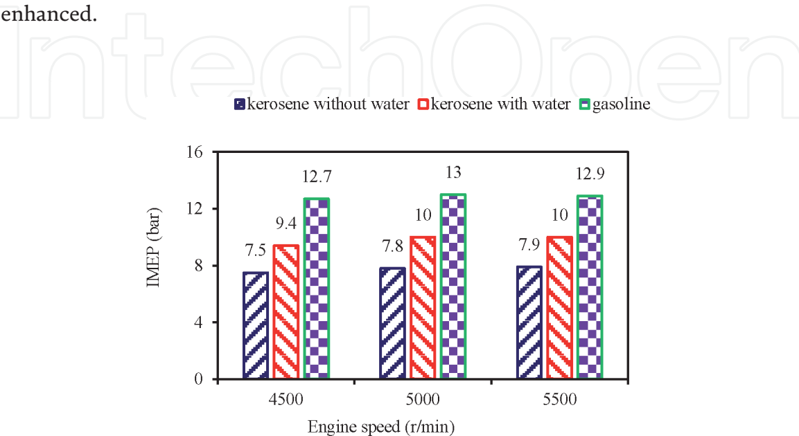
Figure 15. Maximum improvements of the IMEP for the engine fuelled with kerosene together with water injection.
