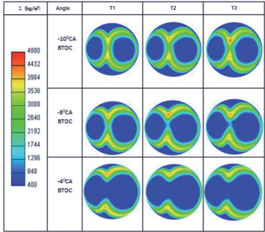
Figure 5. Results of flame surface density with different water injection times.
