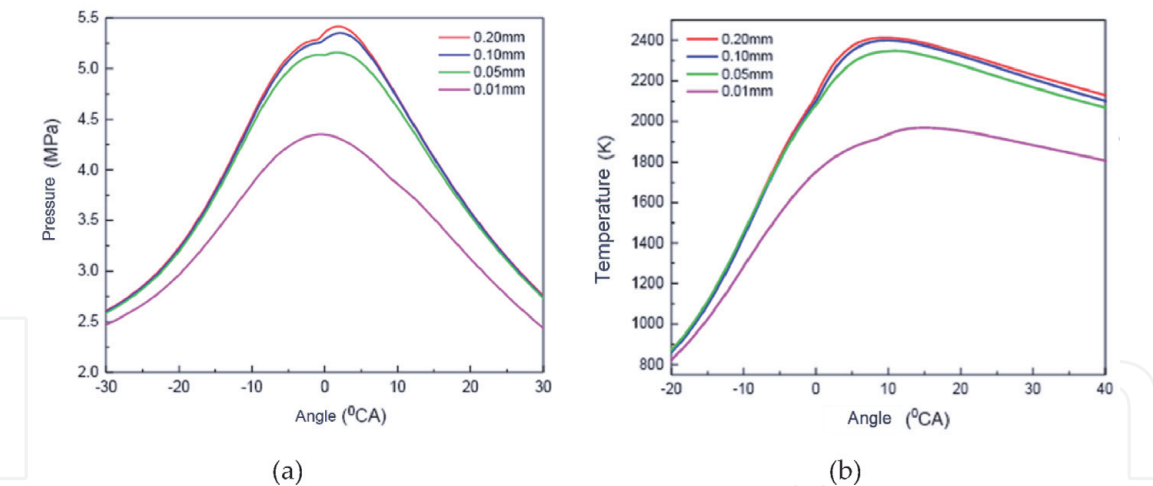
Figure 7. Results of the in-cylinder pressure (a) and temperature (b) with different initial water droplet diameters.
