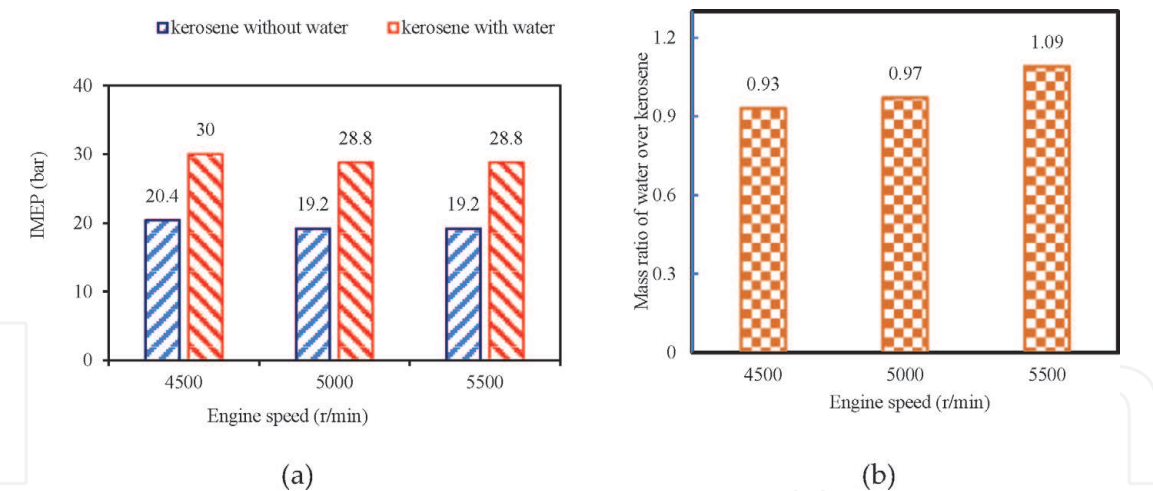
Figure 14. Results for the maximum amount of injected kerosene with/without water injection under different engine speeds (a) and the mass ratio of water over kerosene (b).
