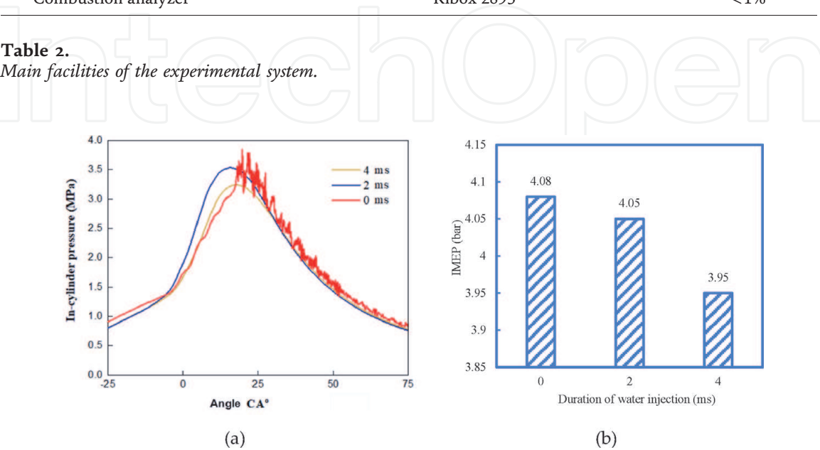
Figure 13. Results for the in-cylinder pressure (a) and IMEP (b) with different water injection durations.
