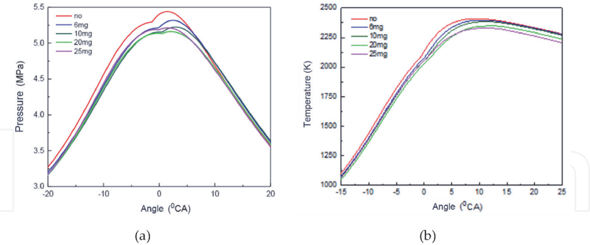
Figure 9. Results of the in-cylinder pressure (a) and temperature (b) with different amounts of water injection.
