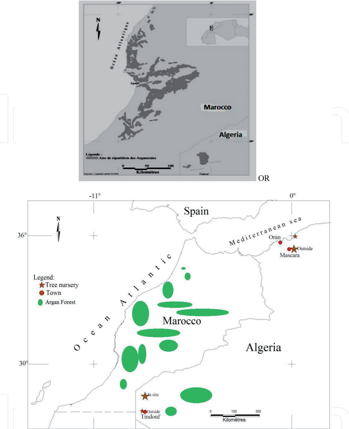
Figure 1. Distribution of the argan tree in Tindouf and northwest Africa [7].
