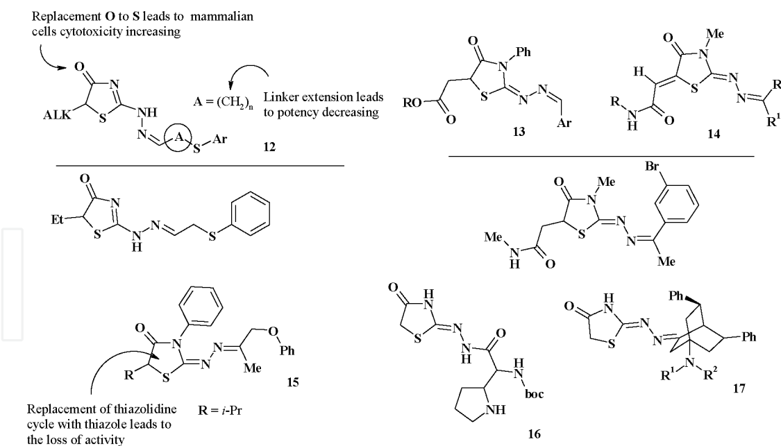
Figure 10. 4-Thiazolidinone-hydrazones as trypanocidal agents.
