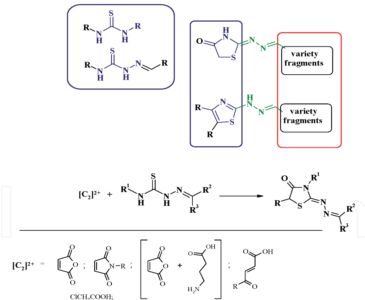
Figure 9. 2-Hydrazono-4-thiazolidinone synthesis.
