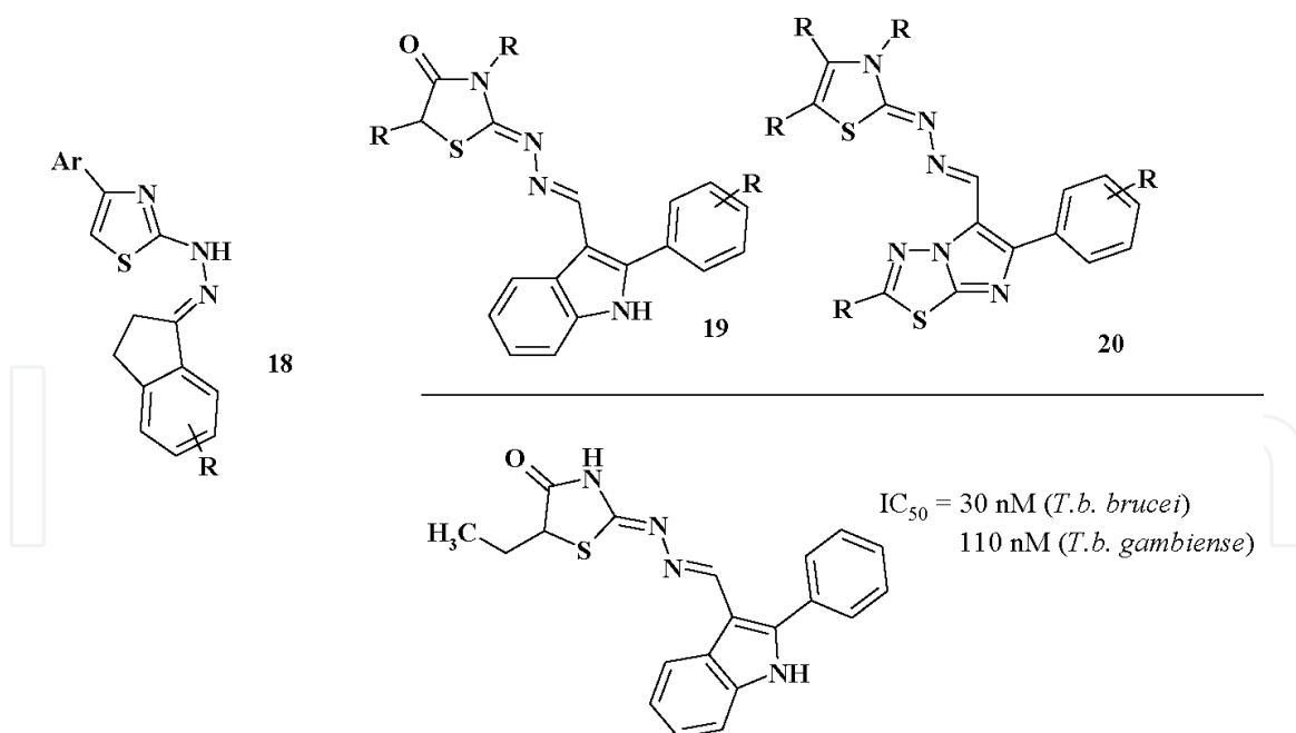
Figure 11. Thiazolidinone-indanone/indole/imidazothiadiazole hybrids.
