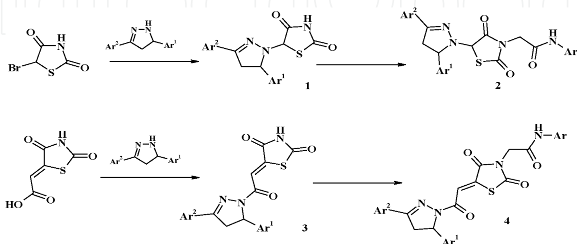
Figure 3. Thiazolidinone-pyrazoline conjugate synthesis.
