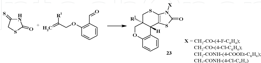
Figure 15. Chromeno-thiopyrano-thiazolidinones as trypanocidal agents.
