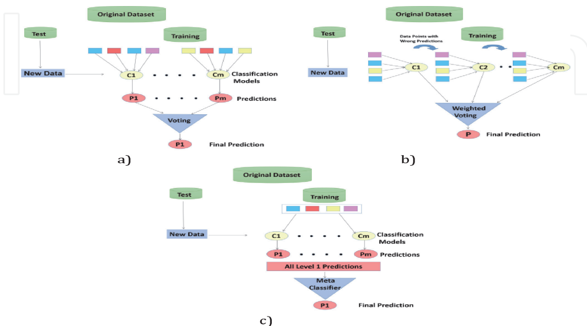
Figure 3. Common ensemble learning methods: (a) Bagging, (b) boosting, (c) stacking.
