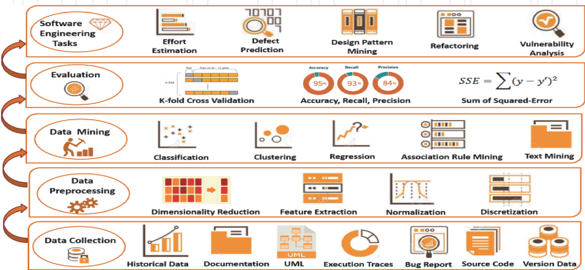
Figure 2. KDD process for software engineering.
