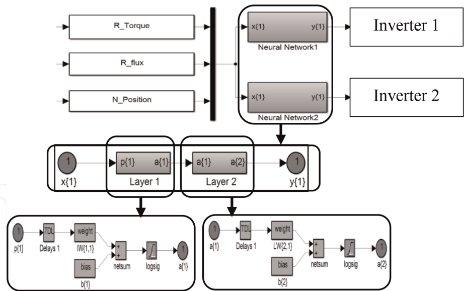
Figure 4. Selection table based on neuron network.
