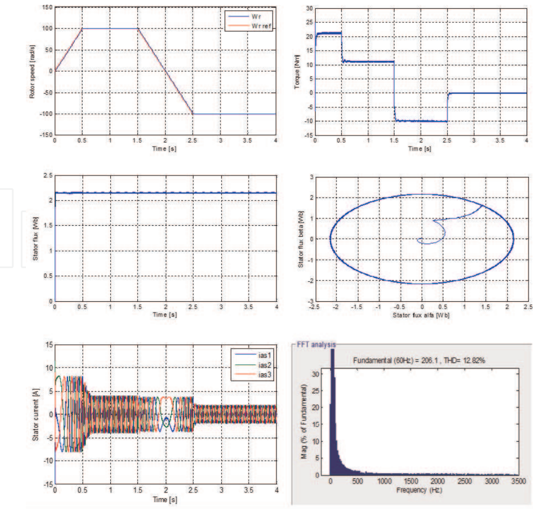
Figure 6. Simulation results of real and estimated speed, torque, flux, and current of five-level DTC-ANN.
