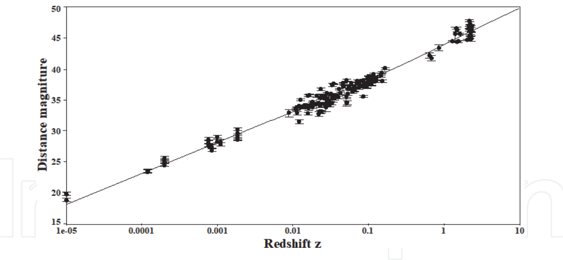
Figure 2. Diagram of a pseudo-H-routine regression using all 156 HII and GEHR data. The centre line is the best fit of the \Lambda CDM model with H_0 fixed at 70.9 \text{ km s}^{-1} \text{ Mpc}^{-1} . Note the abscissa is \log_{10} format to better present nearby emissions.
