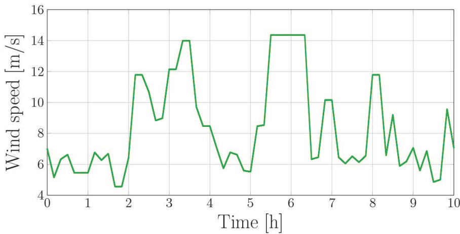
Figure 10. Variation of wind speed with respect to time [14].
