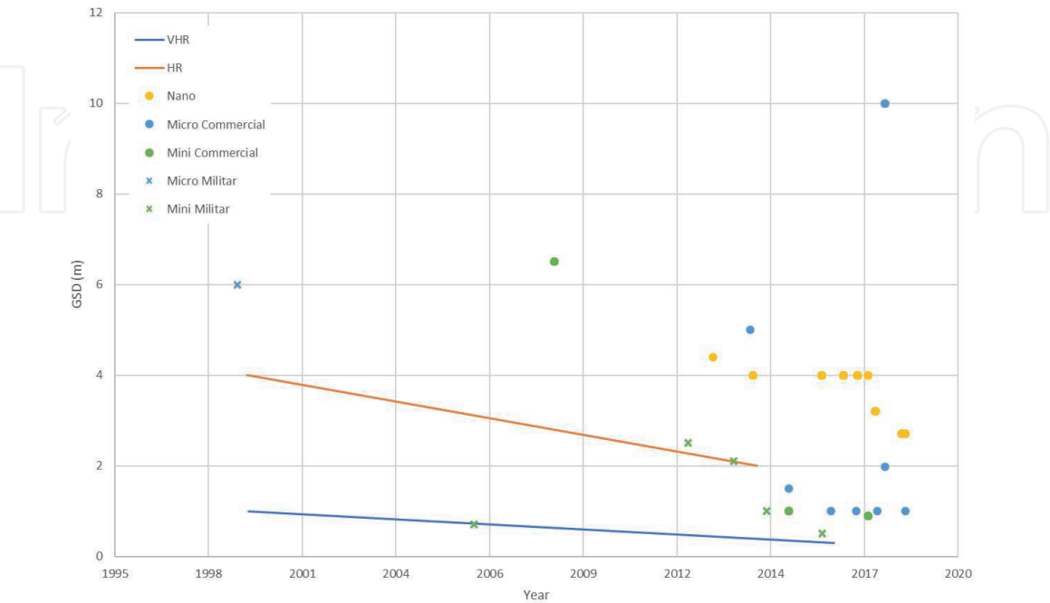
Figure 3. Evolution of EO satellite GSD during the period 1999–2018 (own elaboration).
