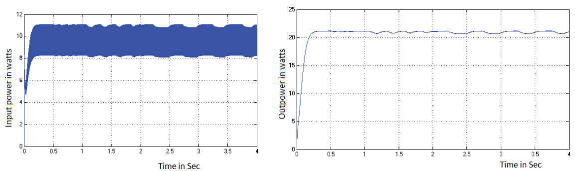
Figure 8. Total input power = 12 W and dual KY converter output power = 22 W.
