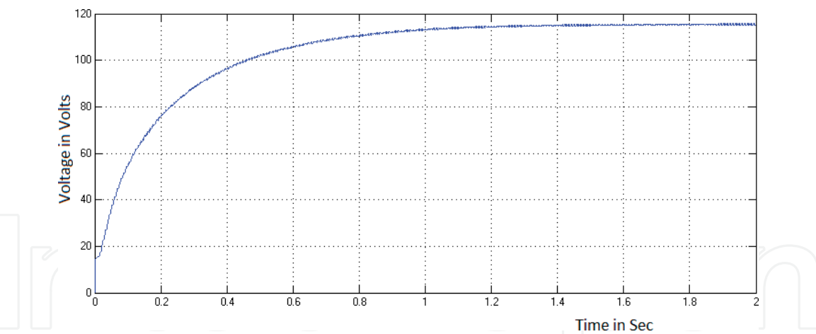
Figure 7. Dual KY boost converter output voltage is 110 V.
