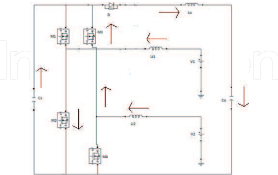
Figure 6. Mode 2 operation of a dual KY boost converter.
