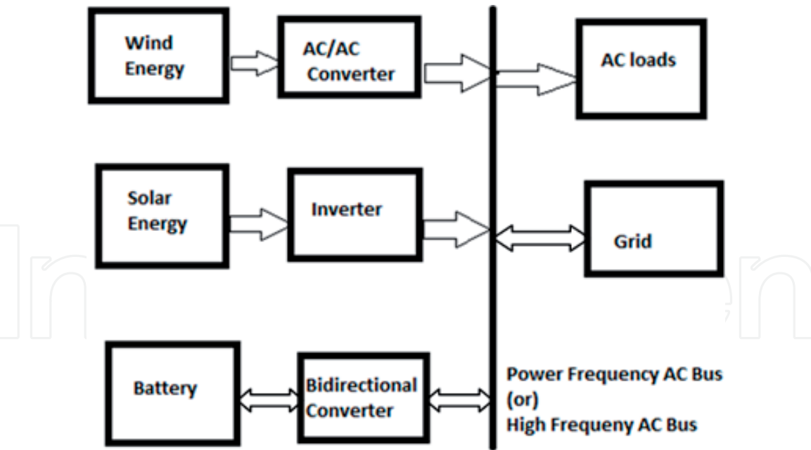
Figure 2. Block diagram of an AC-coupled integration system.
