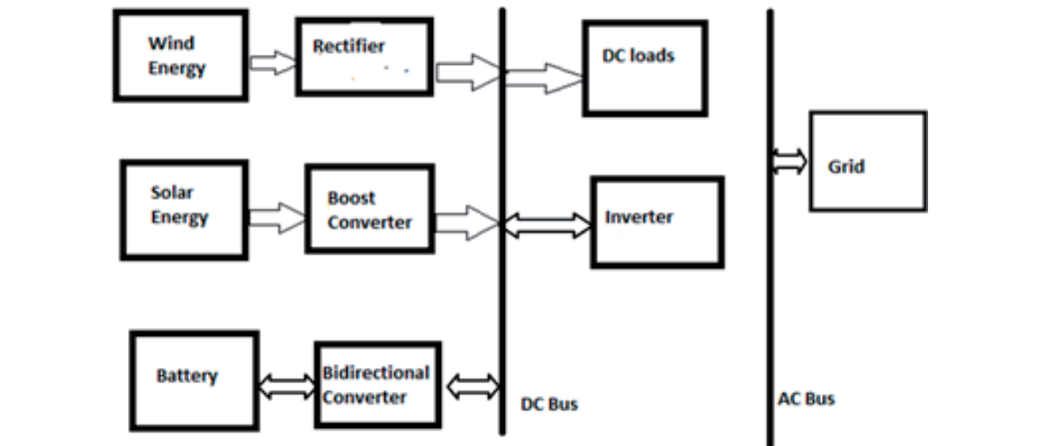
Figure 3. Block diagram of a hybrid-coupled integration system.
