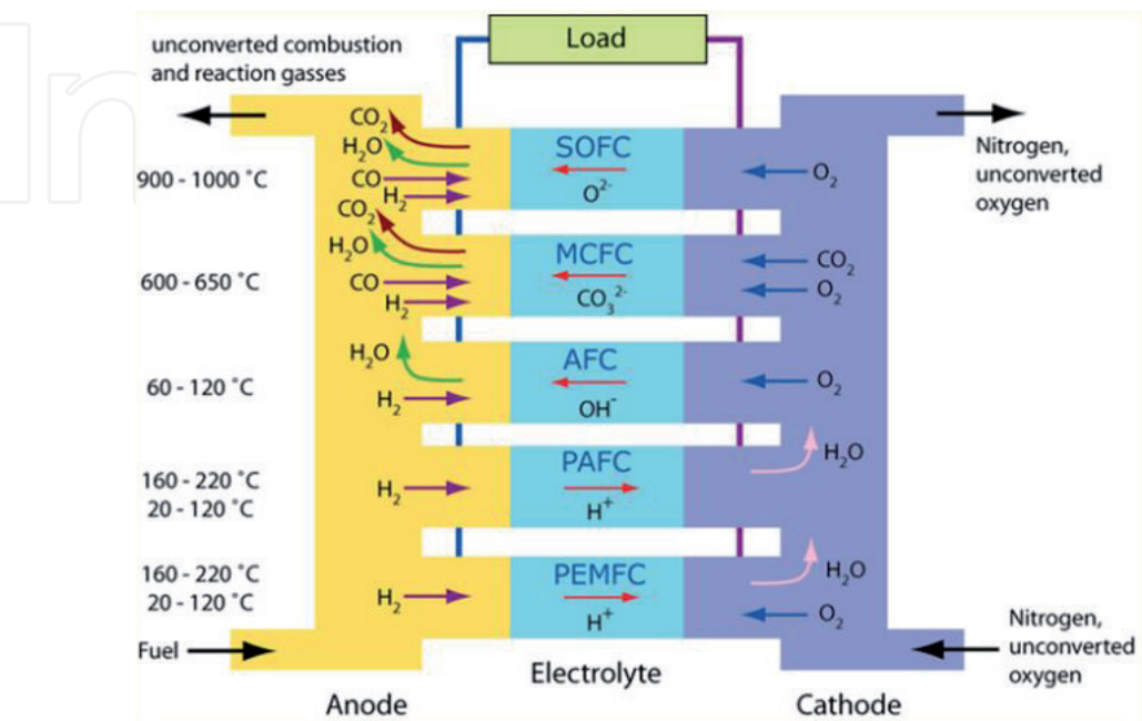
Figure 1. Fuel cells structures and operation temperatures [10, 11].
