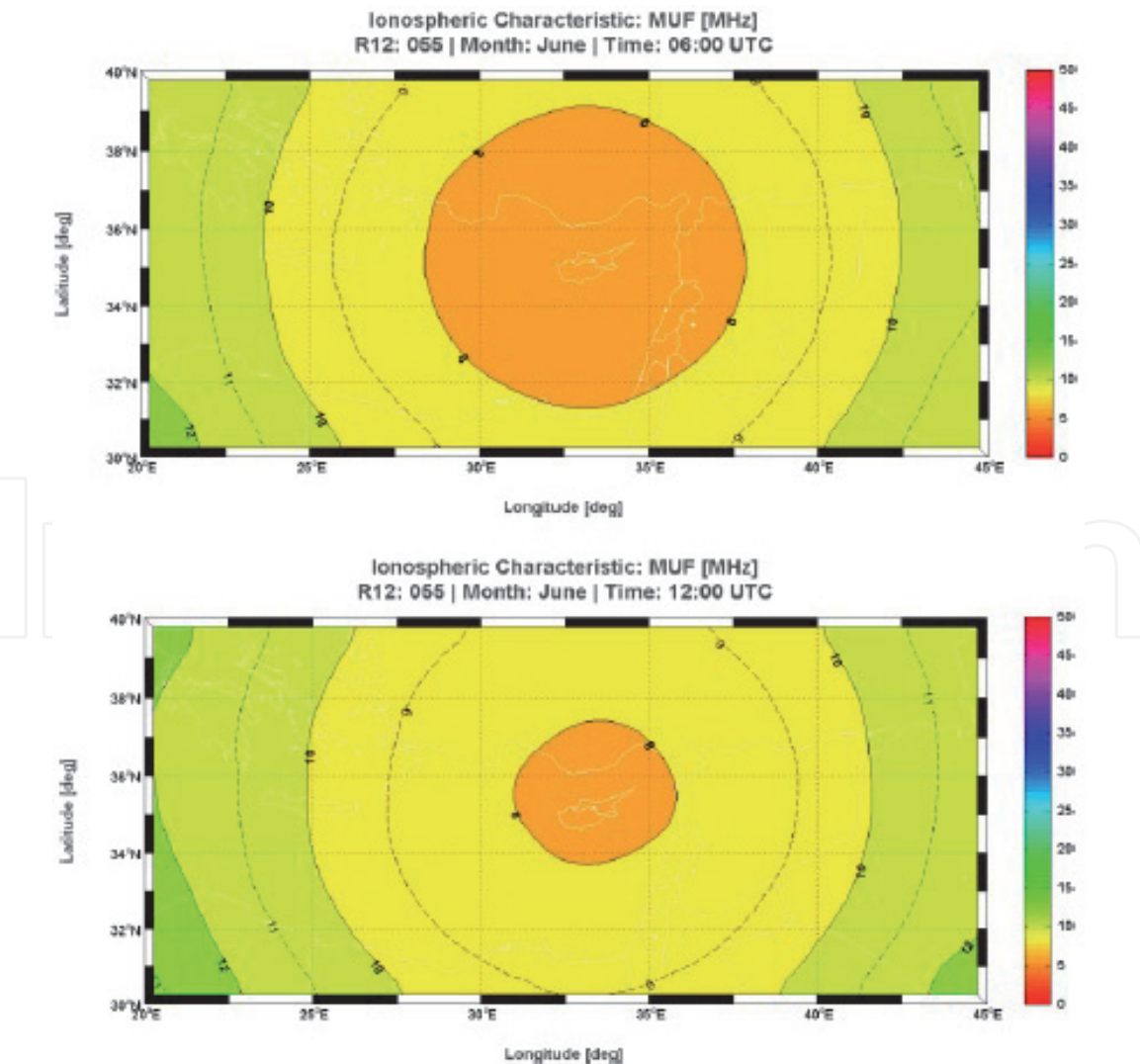
Figure 12. Example of long-term maps of MUF over the eastern part of the Mediterranean Sea predicted by SIRM for the Cyprus Ionospheric forecasting service.
