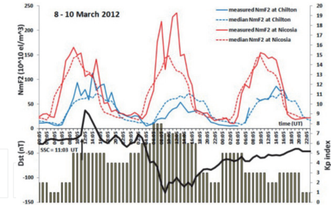
Figure 5. Time variations in Dst and Kp geomagnetic indices and NmF2 at the Chilton (51.6° N, 358.7° E) (blue solid and dashed curves) and at Nicosia (35.1° N, 33.3° E) ionosonde stations (red solid and dashed curves) during the ionospheric storm period of 8–10 March 2012.
