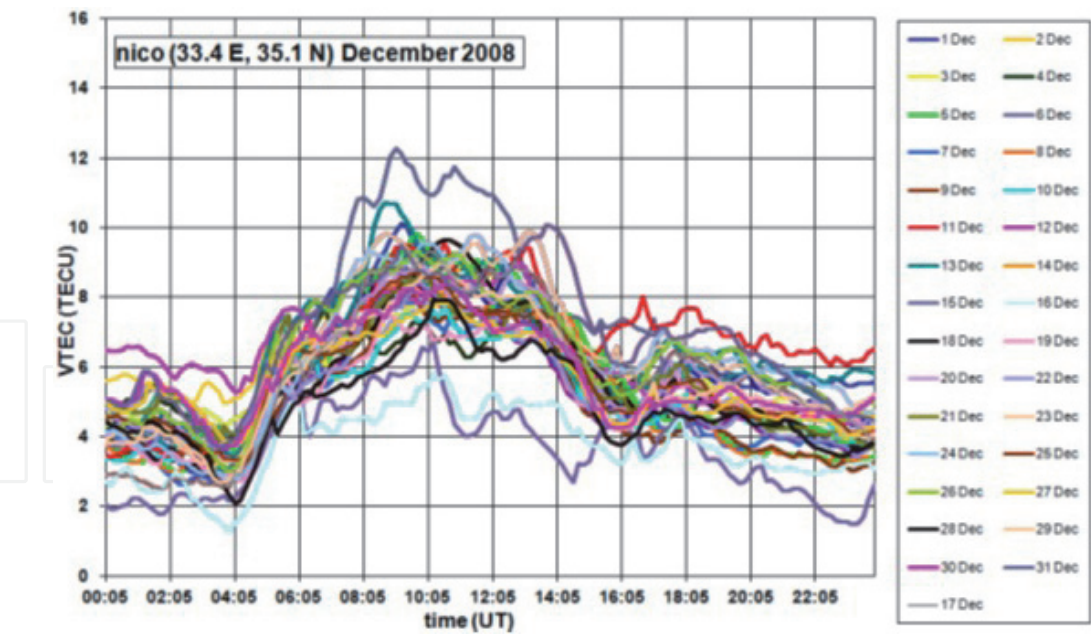
Figure 4. Plot of the day-to-day vertical total electron content VTEC variability at the nico GNSS station over temporal scales from 10 minutes to 1 month during absolute solar minimum in December 2008 with the monthly mean of the daily sunspot number R_i = 0.8 .
