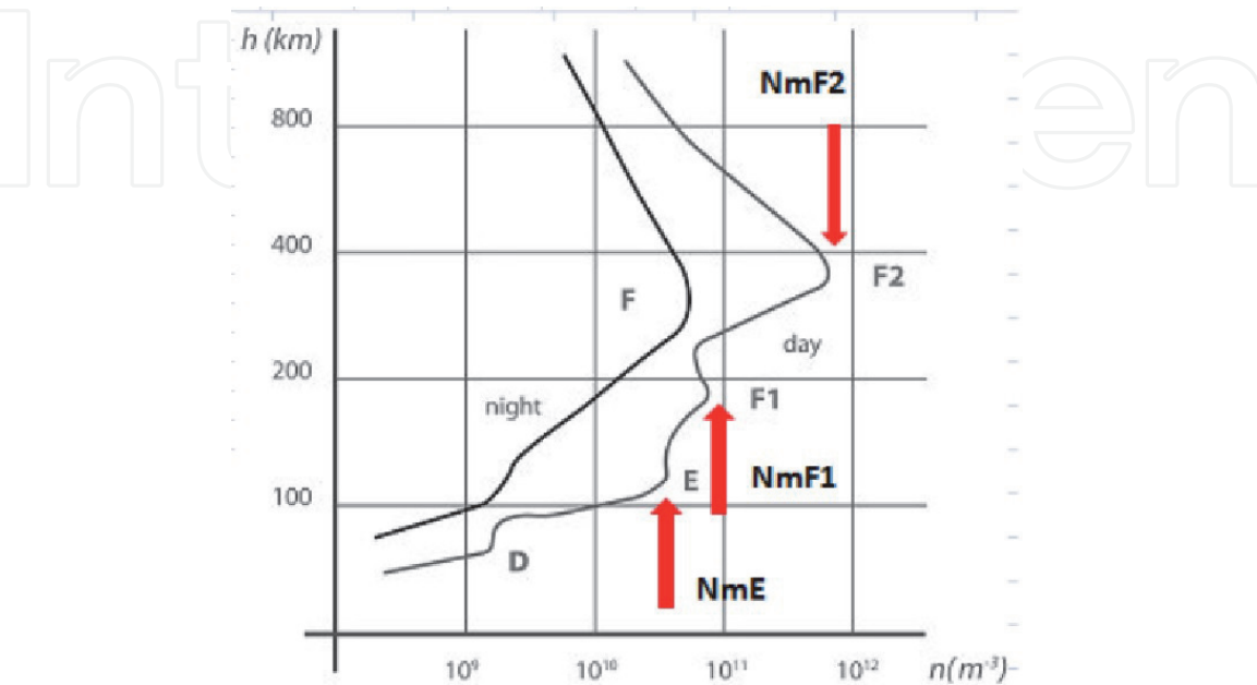
Figure 2. Diurnal and nocturnal ionospheric N(h) profile representing electron density as a function of height.
