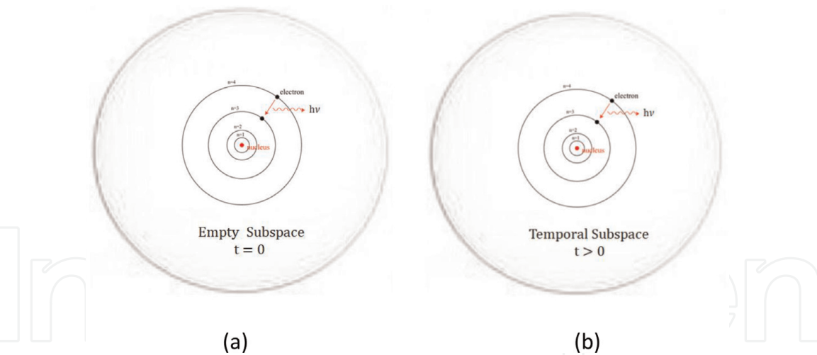
Figure 7. Physical realizable paradigm (a) shows a Bohr atom situated within an empty space, which is “not” a physical realizable model, and (b) shows a Bohr atom situated within a temporal subspace, which is a physical realizable model.
