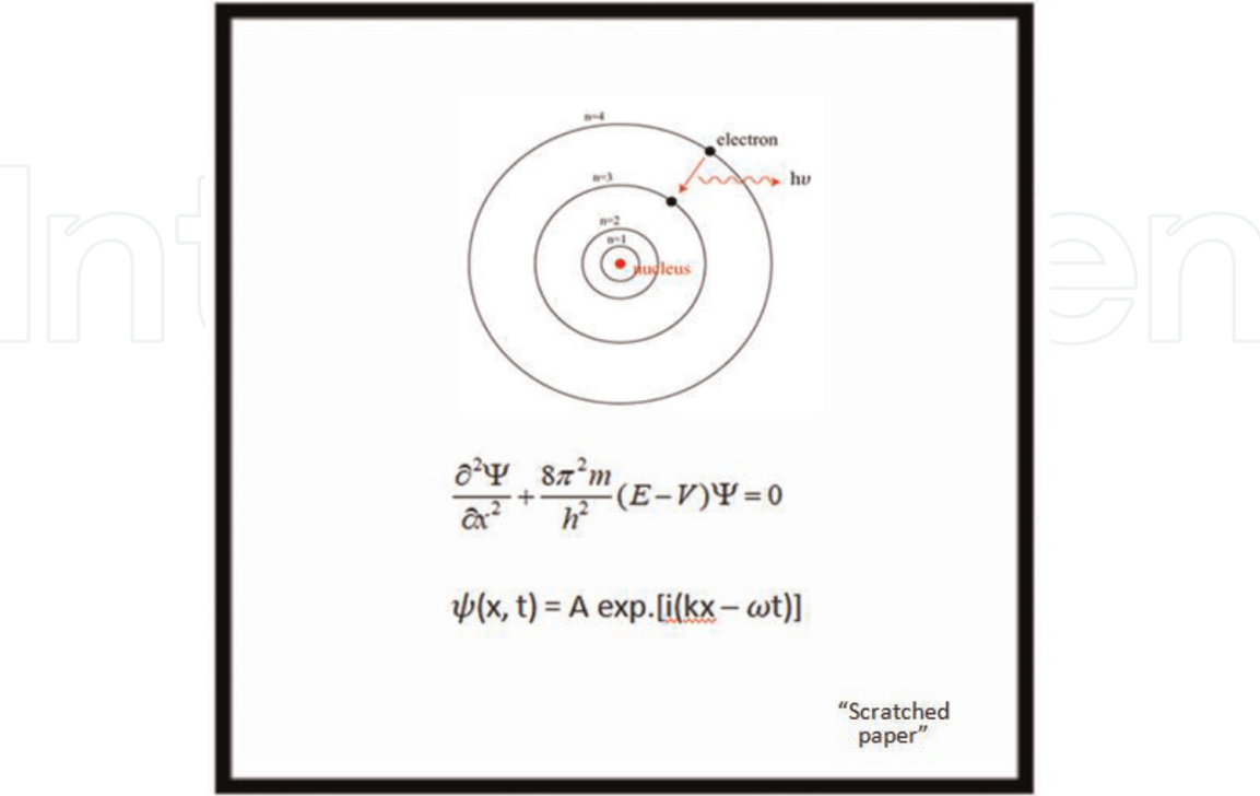
Figure 3. A sample piece of “scratch paper” shows an atomic model with a couple of equations in it.
