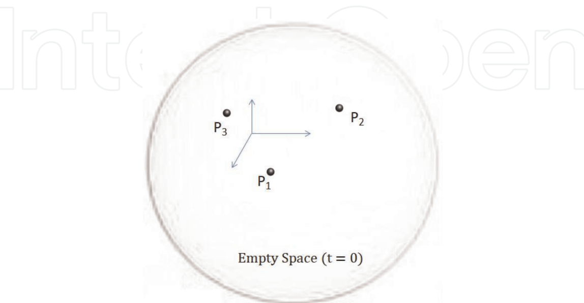
Figure 10. Three separated particles are situated within an empty subspace in different locations. Notice it is a virtual paradigm since substance cannot exist within an empty space.
