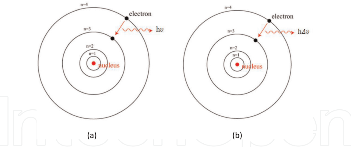
Figure 8. (a) A conventional Bohr Atomic model and (b) the same Bohr model, except the quantum state energy is presented by a band-limited notation h\Delta\nu .
