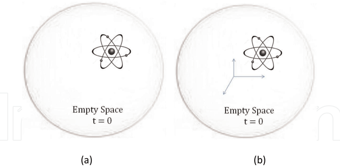
Figure 2. A set of atomic models embedded within virtual empty subspaces (a) shows a singularity approximated atomic model is situated within an empty space, which has no coordinate system, and (b) shows an atomic model is embedded within an empty space that has a coordinate system drawn into it.
