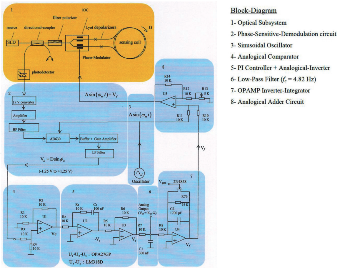
Figure 8. Closed-loop IFOG scheme with sinusoidal BIAS and serrydyne FEEDBACK phase modulations, see Ref. [25] (below, in the inset, the block-diagram definition).
