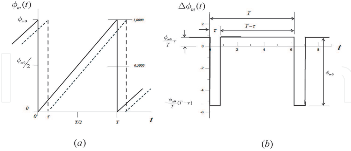
Figure 9. Serrodyne-wave phase modulation: (a) serrodyne-wave applied to PM with amplitude \phi_{m0} and period T and (b) effective phase-difference \Delta\phi_m(t) as a function of time.
