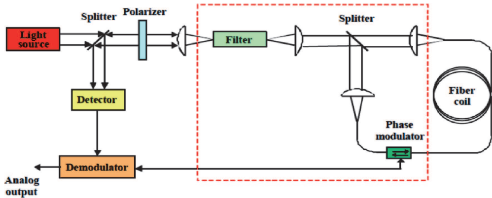
Figure 3. Complete bulk-optics fiber-optic gyro open-loop configuration.
