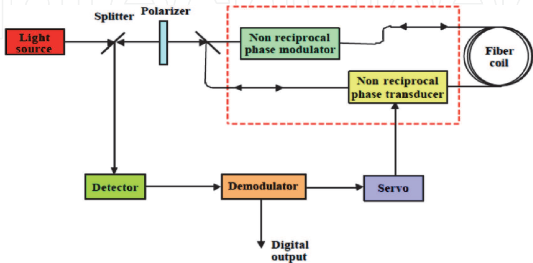
Figure 4. Typical closed-loop IFOG configuration.
