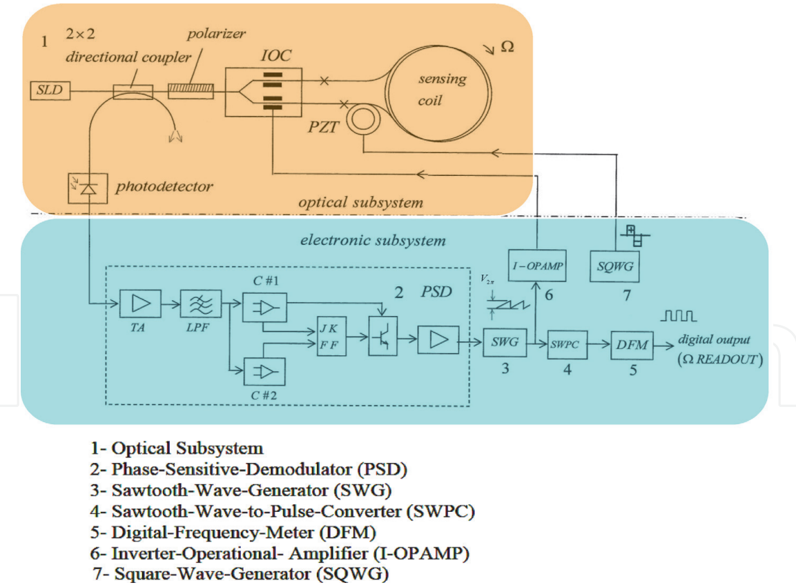
Figure 6. Closed-loop IFOG scheme with square-wave BIAS and serrodyne FEEDBACK phase modulations (below, in the inset, the block-diagram definition).
