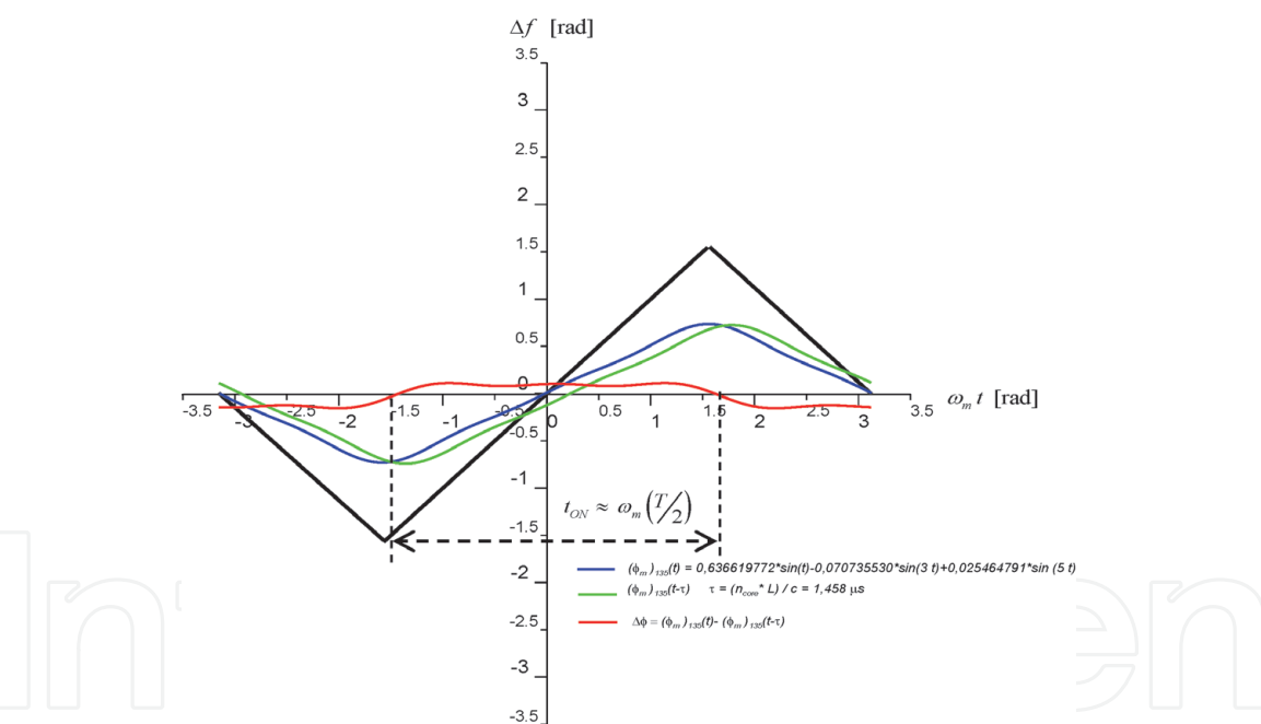
Figure 14. Effective phase-difference modulation of symmetric triangular wave (red-curve) related with its first three harmonic Fourier sums (blue, green) of CCW and CW optical waves, Ref [35].
