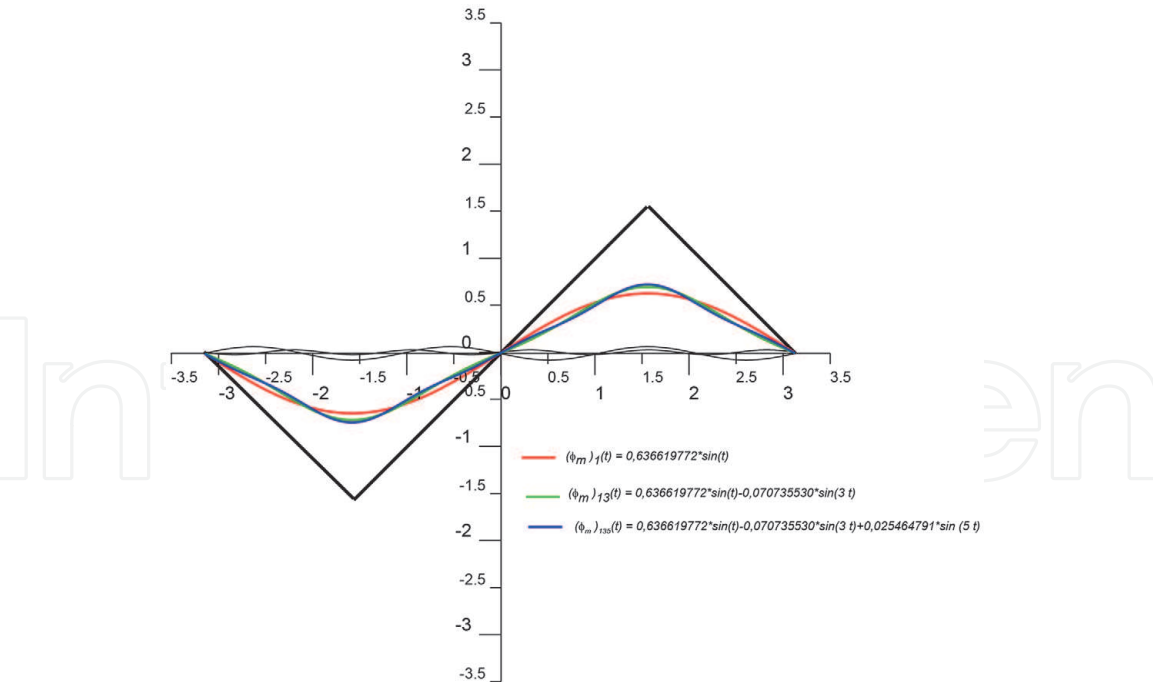
Figure 13. Symmetric triangular wave (in black) with its first three harmonic Fourier sums (red, green, blue), Ref. [35].
