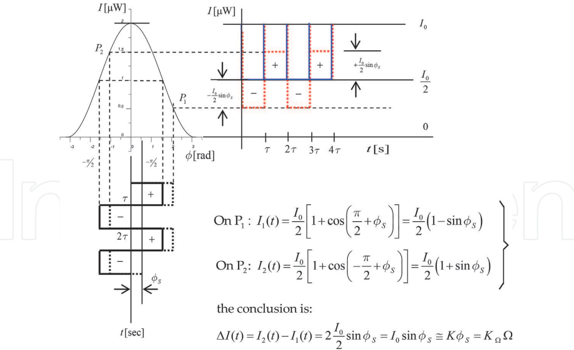
Figure 5. Analysis of the interference response of the gyro with square-wave phase modulation (solid blue curve: zero rotation, dotted red curve: non-zero rotation).
