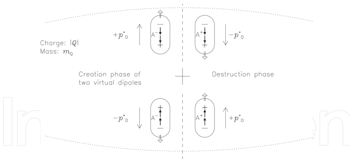
Figure 1. Conceptional presentation of the creation and destruction phases of virtual dipole pairs by a charge and the corresponding momentum vectors of the virtual dipoles (long arrows). The dipoles are assumed to have a spin of S = \pm 2 \times \hbar/2 (short arrows) (Figure 2 of [17]).
