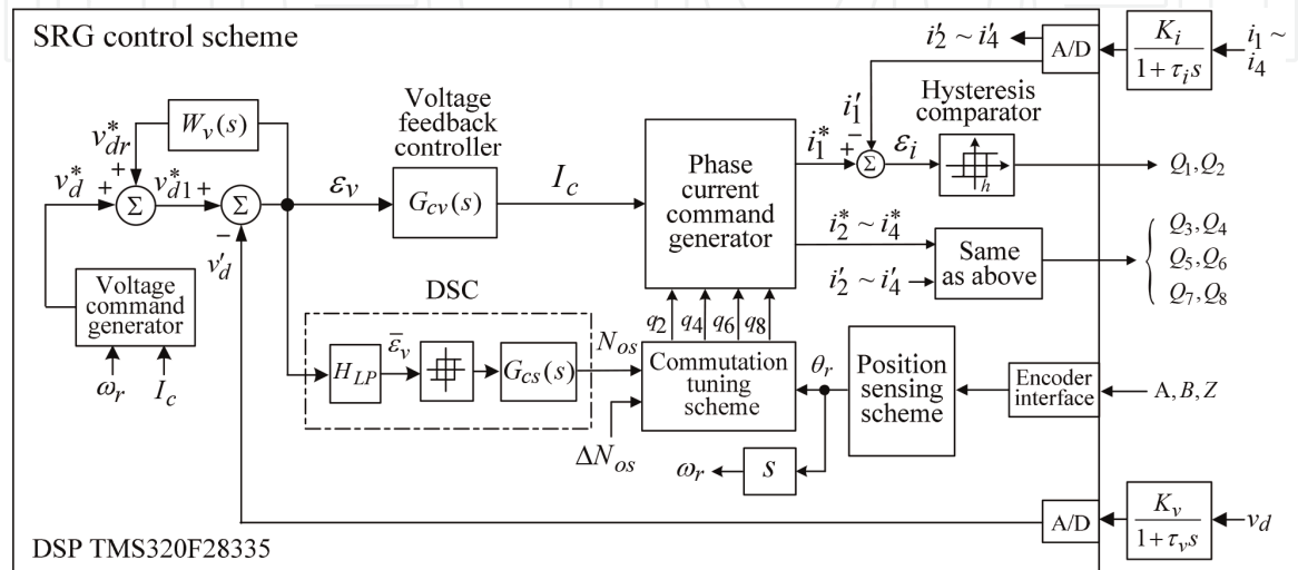
Figure 16. Control scheme of the wind SRG.
