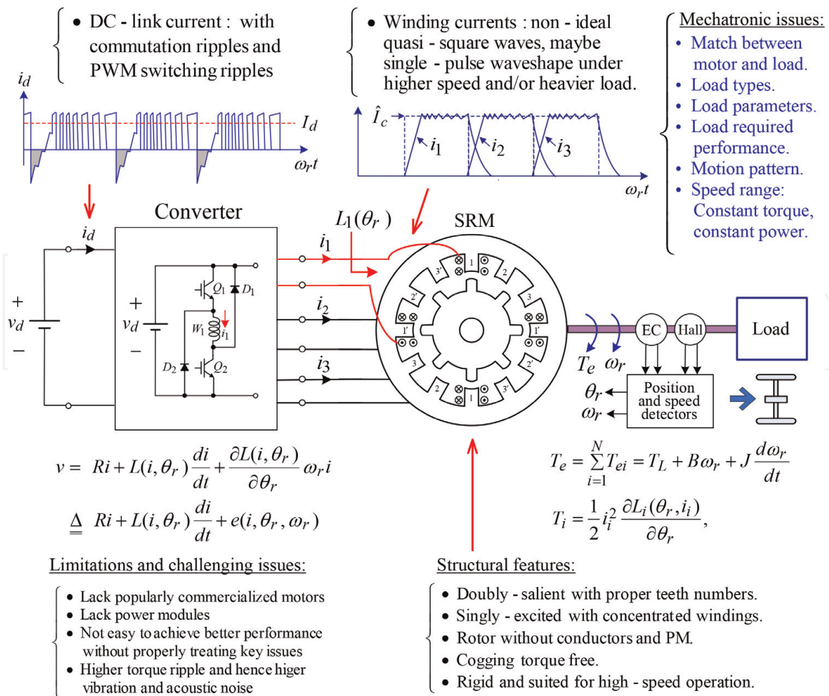
Figure 1. Key features of switched-reluctance machines.
