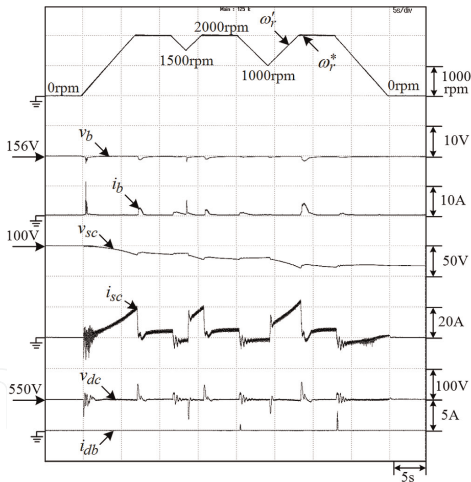
Figure 28. The EV SRM drive powered by battery and SC at V_b = 156\text{ V} , V_{SC} = 100\text{ V} , V_{dc} = 550\text{ V} , R_m = 455\text{ }\Omega .
