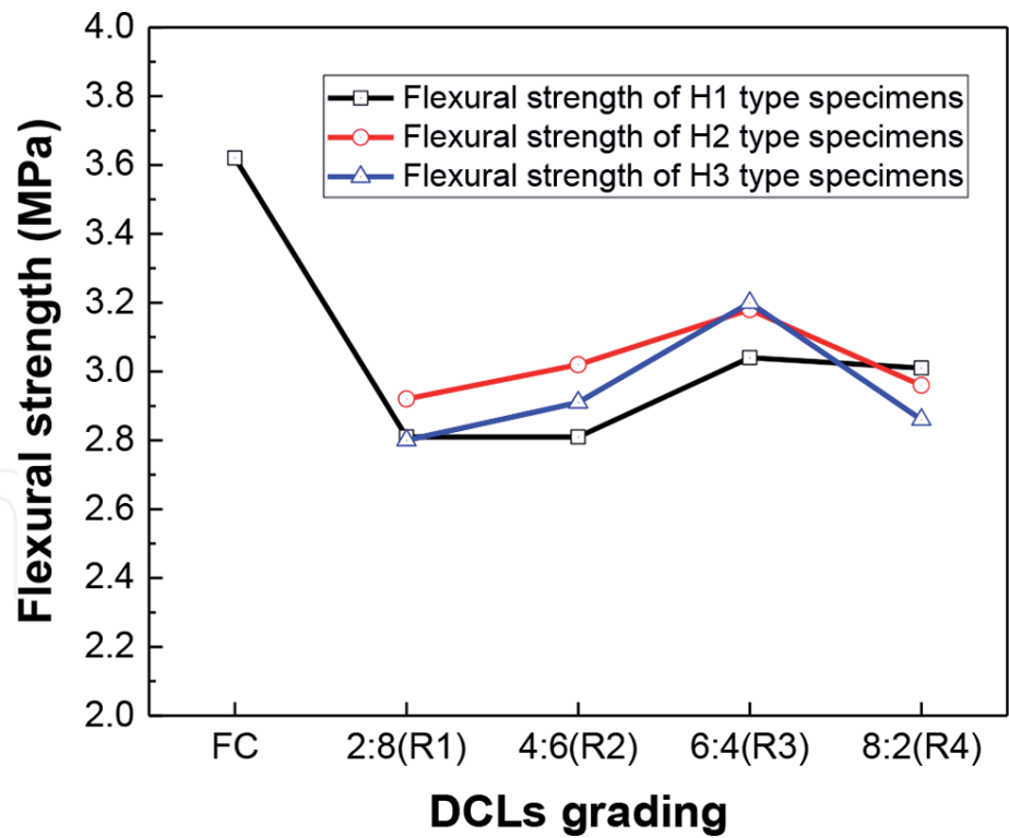
Figure 13. Flexural strength of compound concrete with different gradations of DCLs.
