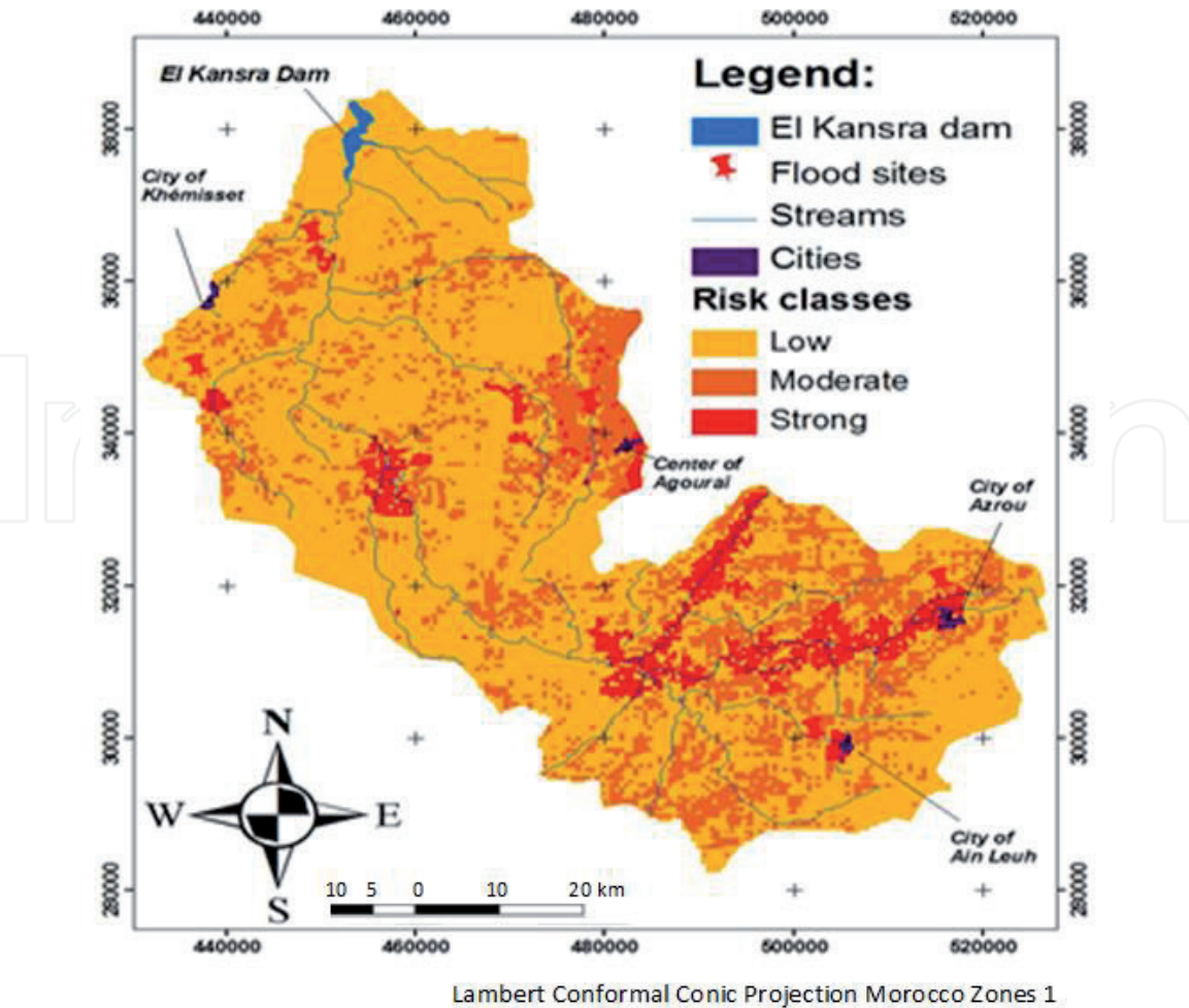
Figure 21. Natural erosion risks.
