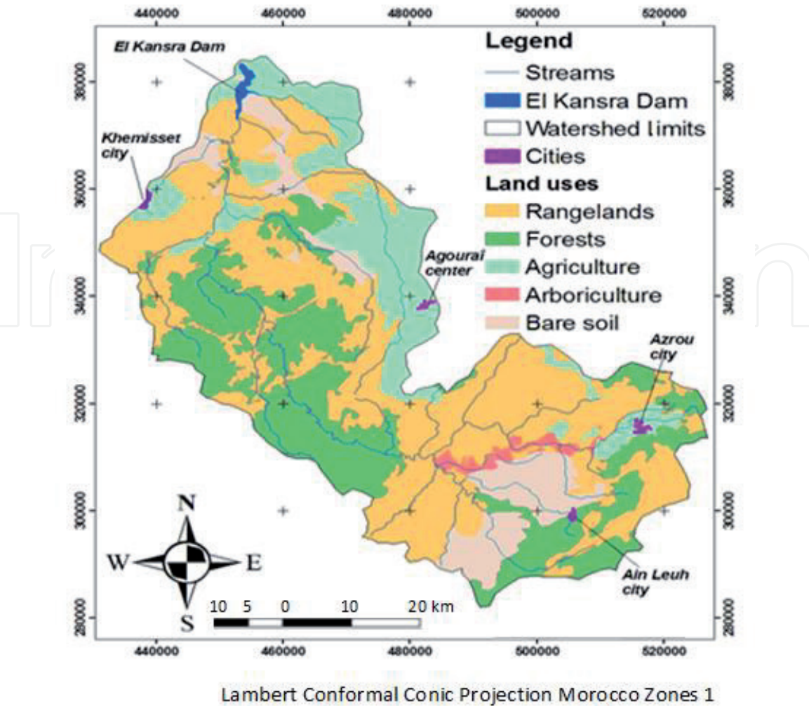
Figure 14. Land use map.
