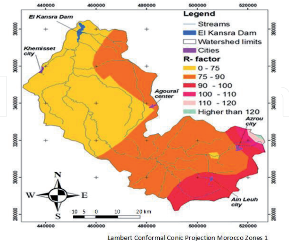
Figure 13. R-factor distribution.
