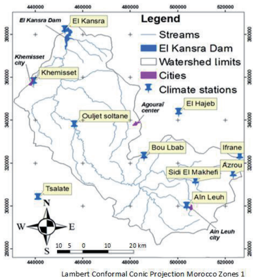
Figure 11. Distribution of climate stations.
