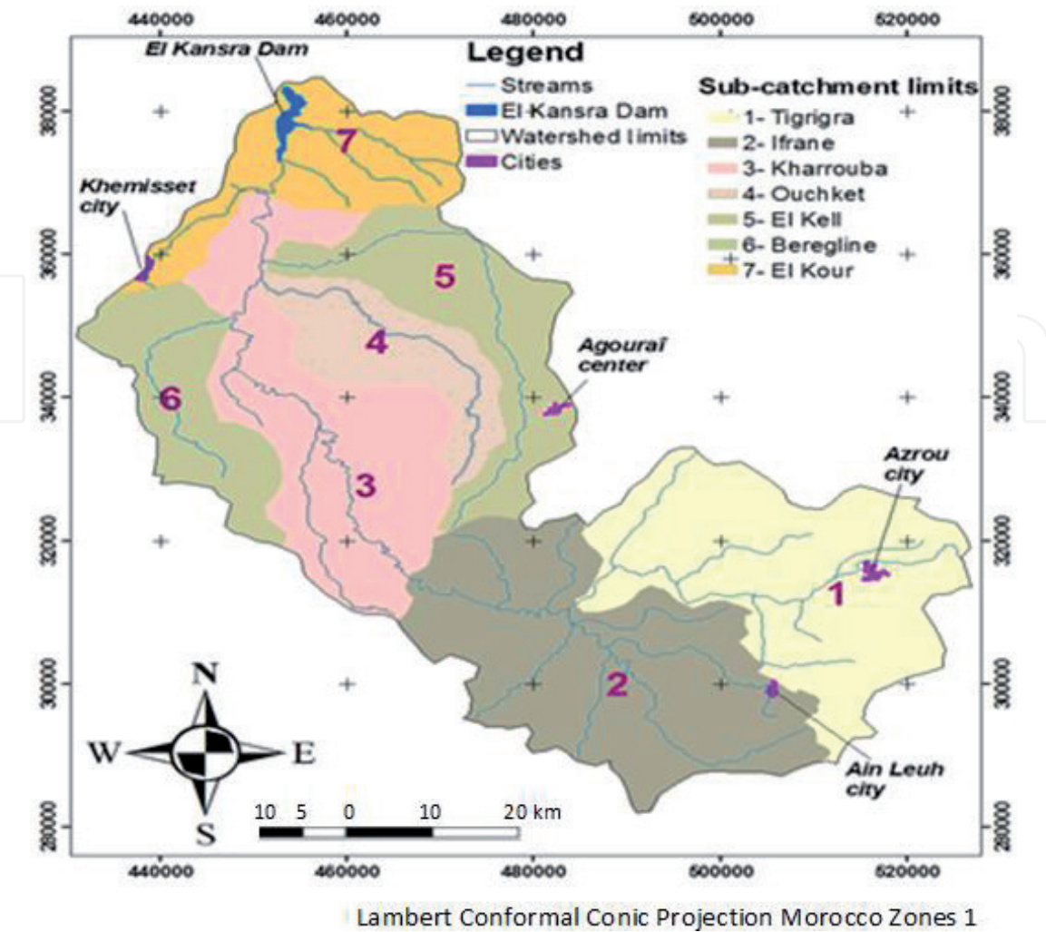
Figure 17. Sub-catchment delimitation.
