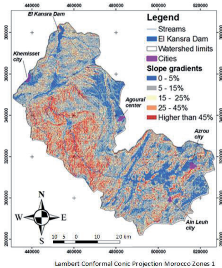
Figure 7. Slope gradient map of the study area.
