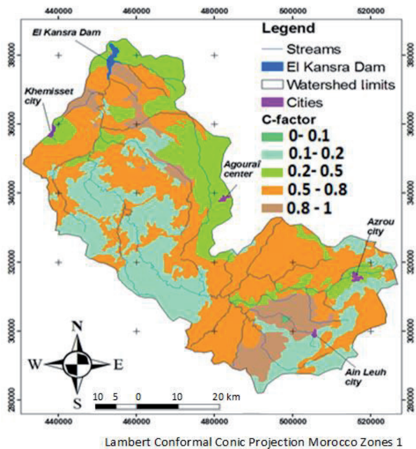
Figure 16. C-factor distribution.
