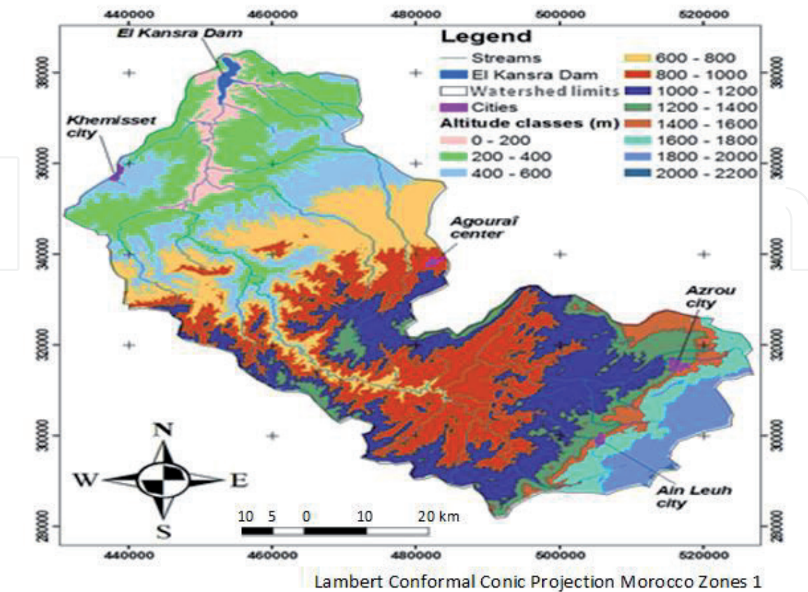
Figure 5. Hypsometric map.
