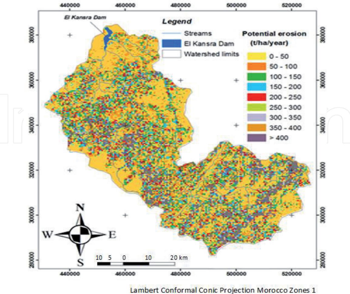
Figure 18. Potential erosion map.
