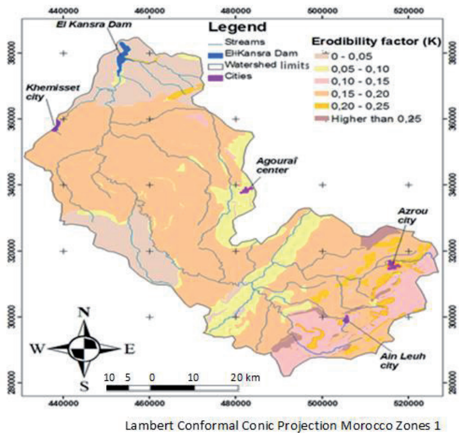
Figure 10. Soil erodibility distribution.
