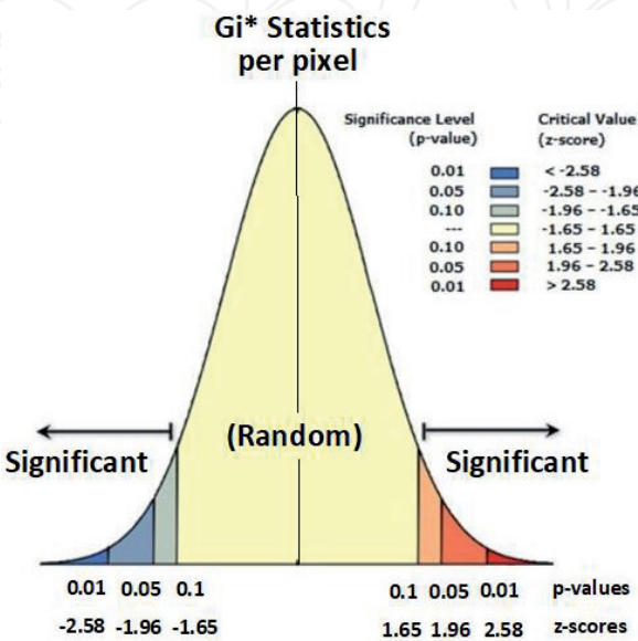
Figure 4. Distribution of spatial autocorrelation indicators (adapted from [18]).
