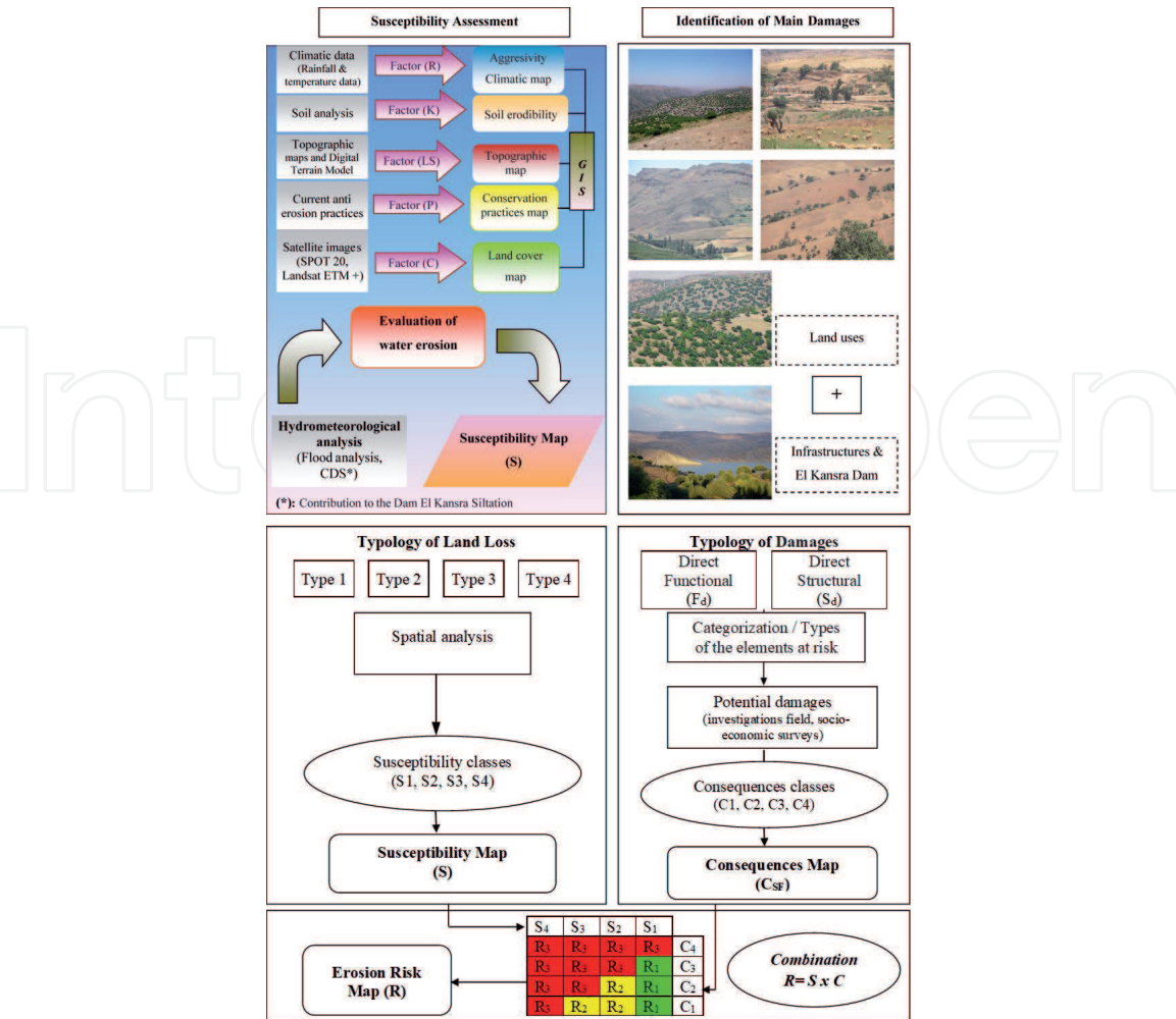
Figure 3. The methodological flowchart to identify priority areas and evaluate soil erosion risk.
