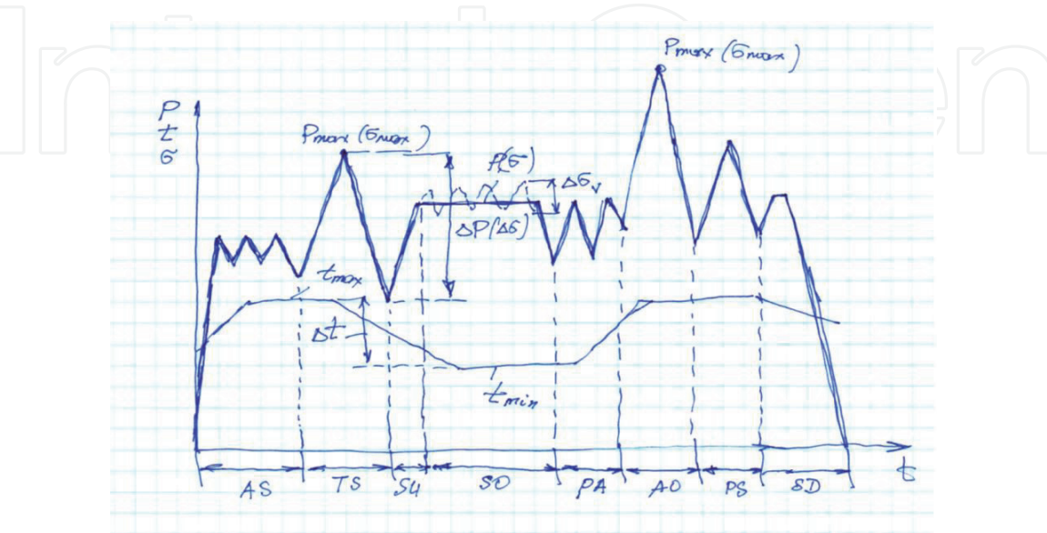
Figure 12. Diagram of operational loads and their basic parameters.
