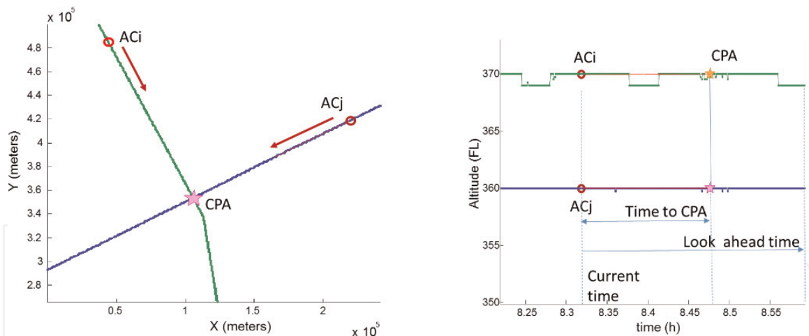
Figure 3. Identification of a conflict from the segmented trajectories (courtesy of Eduardo Garcia).
