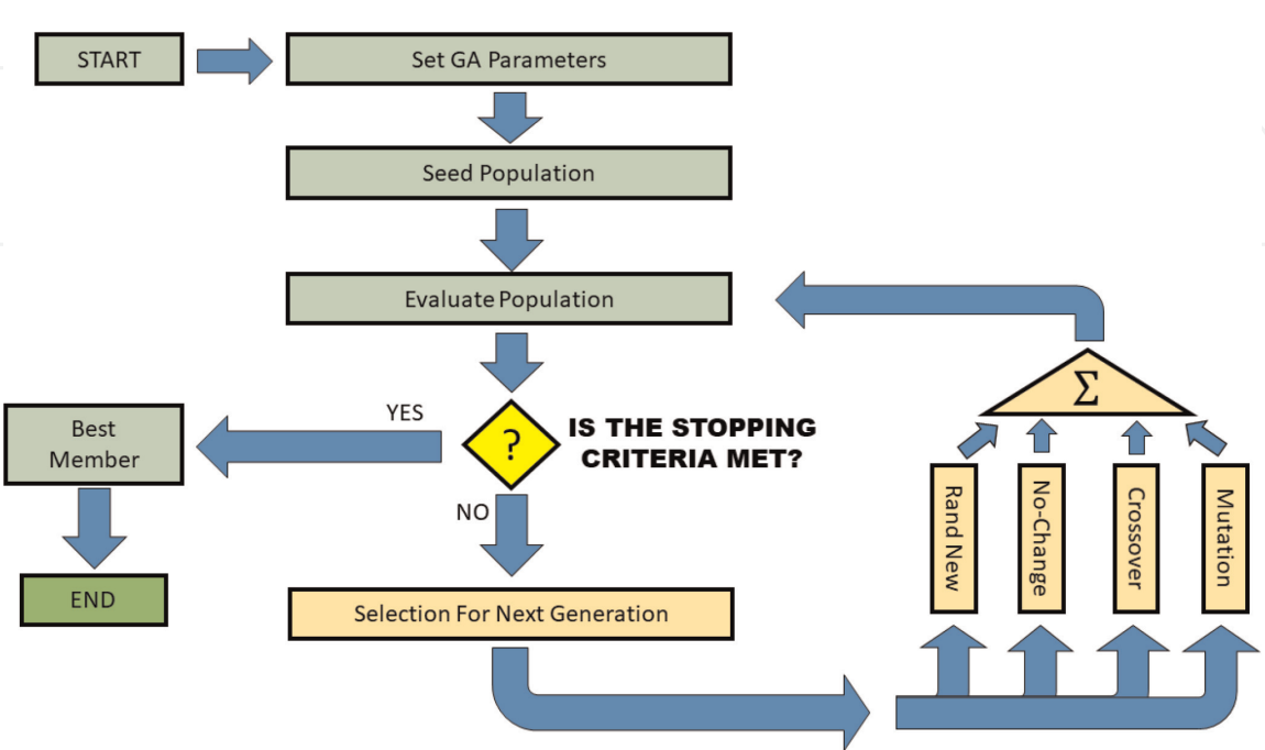
Figure 1. Generic genetic algorithm flow diagram.
