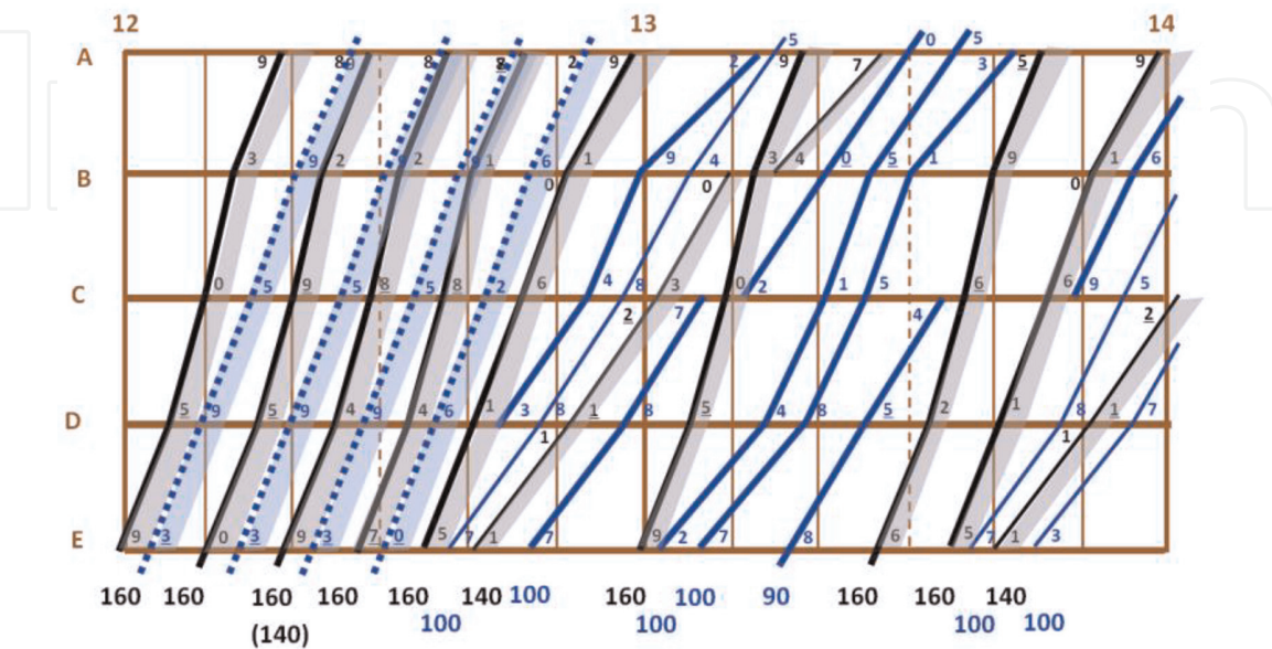
Figure 3. Inability to insert fast freight train paths (Nex) into gaps between express passenger trains (Ex) indicating the occupation time by those paths in a typical mix of train paths on the transit corridor section (numbers below the paths indicate the specified speed for that path).
