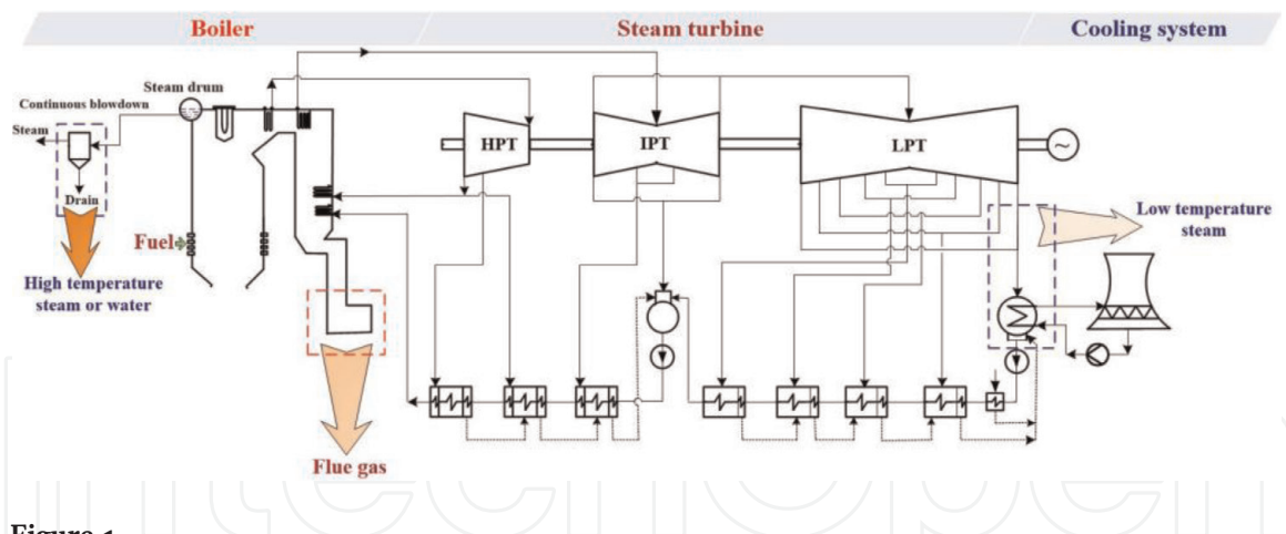
Figure 1. Schematic of the waste heat sources can be recovered by ORCs in a typical coal-fired power unit.
