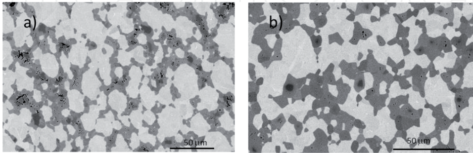
Figure 5. SEM images of TMCs made from composition of 30 vol.% of TiC hot consolidated at (a) 1000°C and (b) 1200°C.
