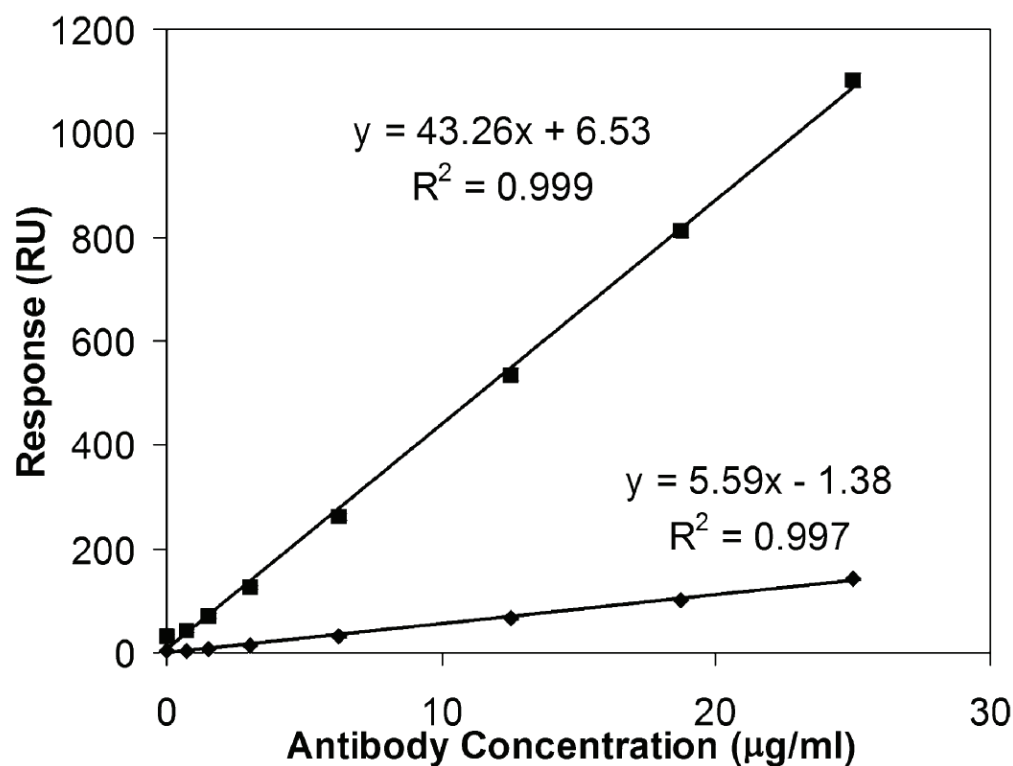
Fig. 4. Plots of SPR response (RU) vs. antibody concentration (μg/mL) for unenhanced mAb only assay (◆) and secondary antibody enhanced assay (■). Reprinted from Analytical Biochemistry, 343, Mitchell, J. S.; Wu, Y.; Cook, C. J.; Main, L. Sensitivity enhancement of surface plasmon resonance biosensing of small molecules. 125-135, 2005, with permission from Elsevier.
